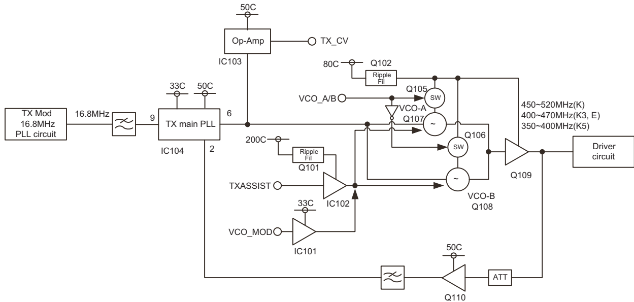
Fig.5 Transmitter main PLL circuit
