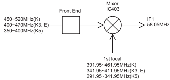
Fig.12 1st-Mixer circuit
