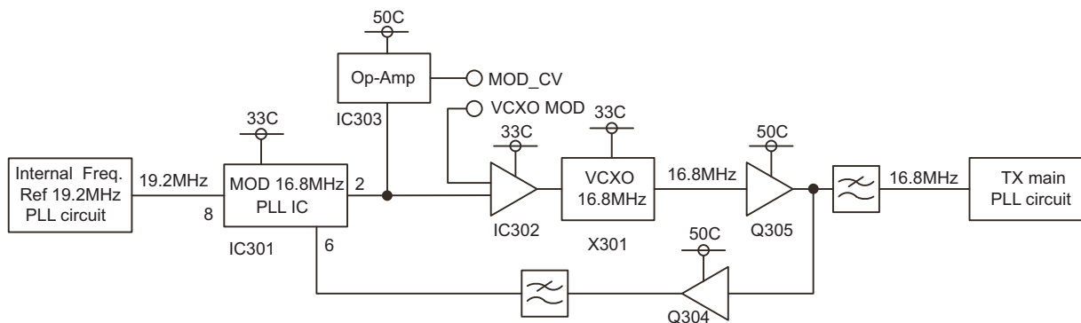
Fig.4 Transmitter Modulation 16.8MHz PLL circuit
