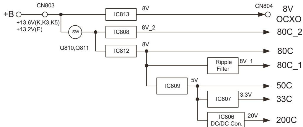
Fig.8 AVR circuit
