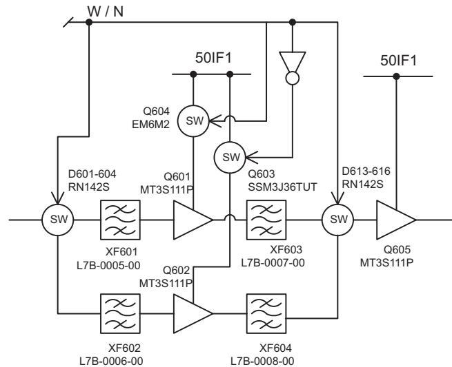
Fig.13 1st-IF circuits
