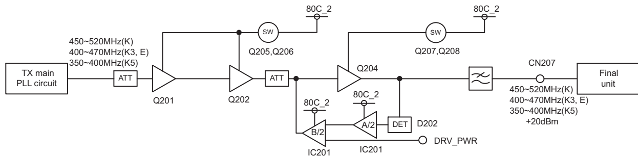
Fig.6 Driver circuit
