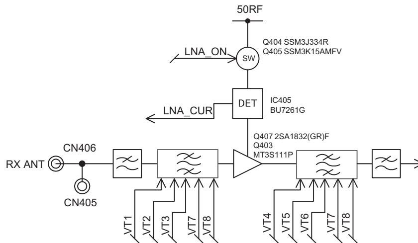
Fig.11 Front-end circuit
