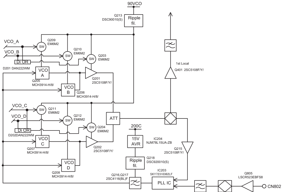
Fig.15 Receiver PLL circuits
