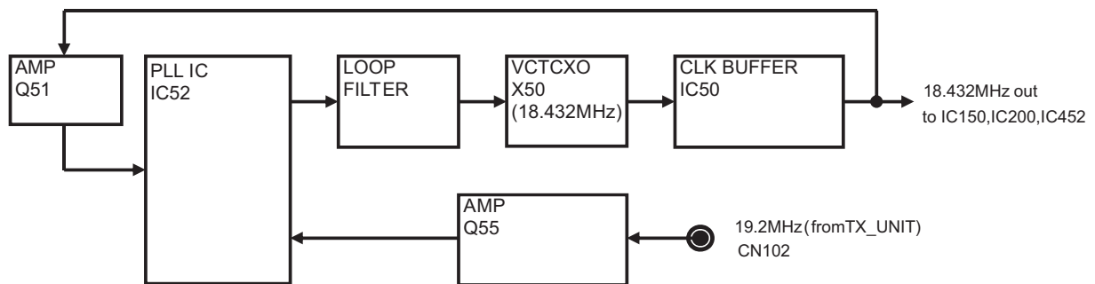
Fig.19 PLL circuit
