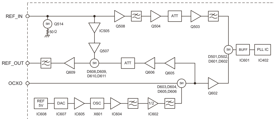
Fig.2 Internal/external reference circuit
