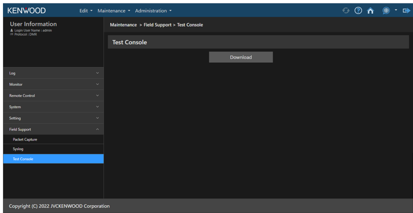
Figure 2-35 Test Console
