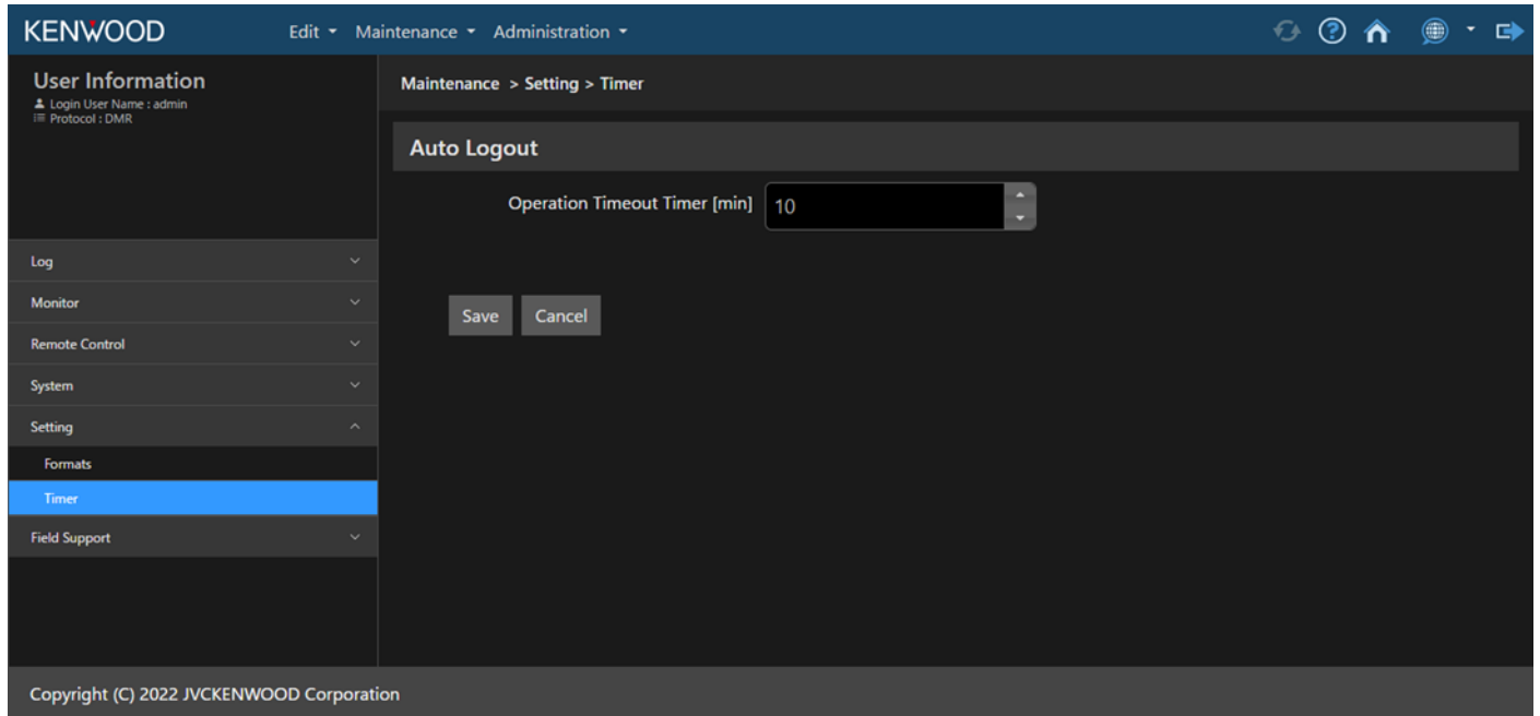
Figure 2-32 Setting > Timer
