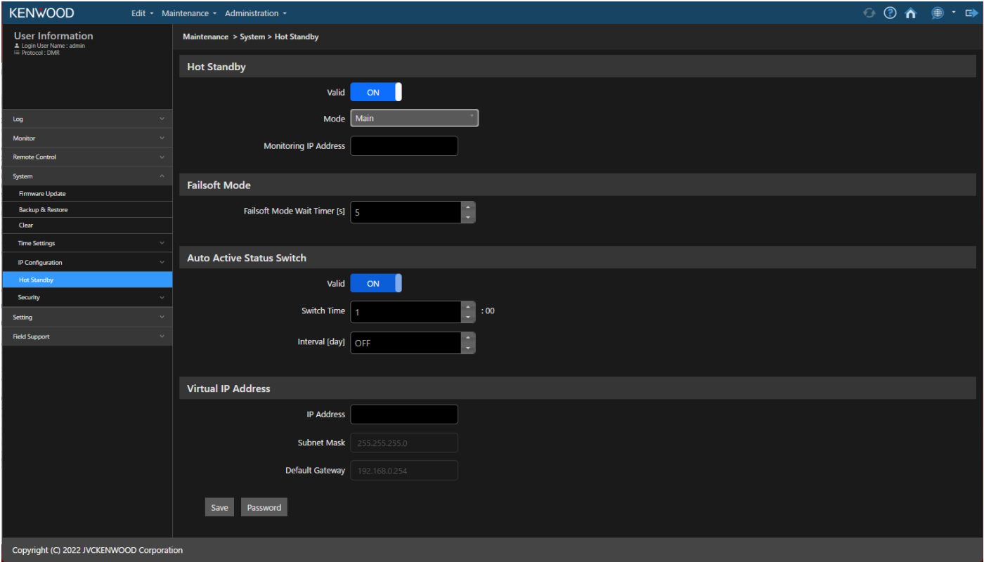
Figure 2-24 Hot Standby
