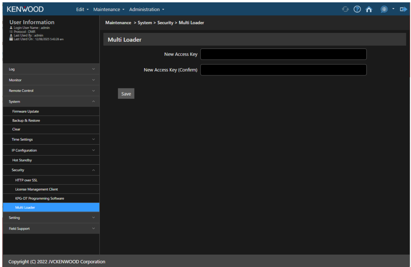
Figure 2-29 Security > Multi Loader
