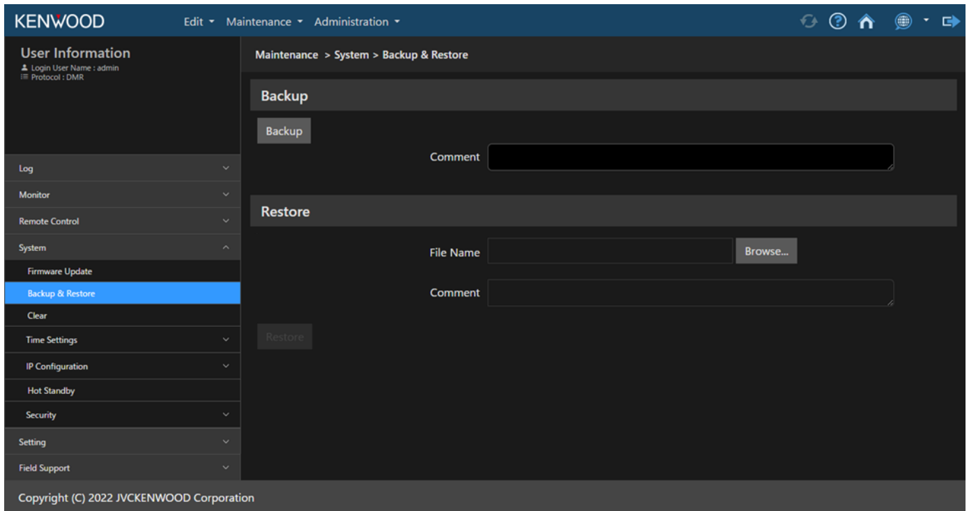
Figure 2-18 Backup & Restore
