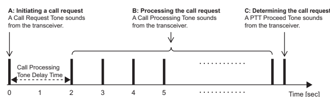
Figure 2-2 Call Request Tone/ Call Processing Tone
