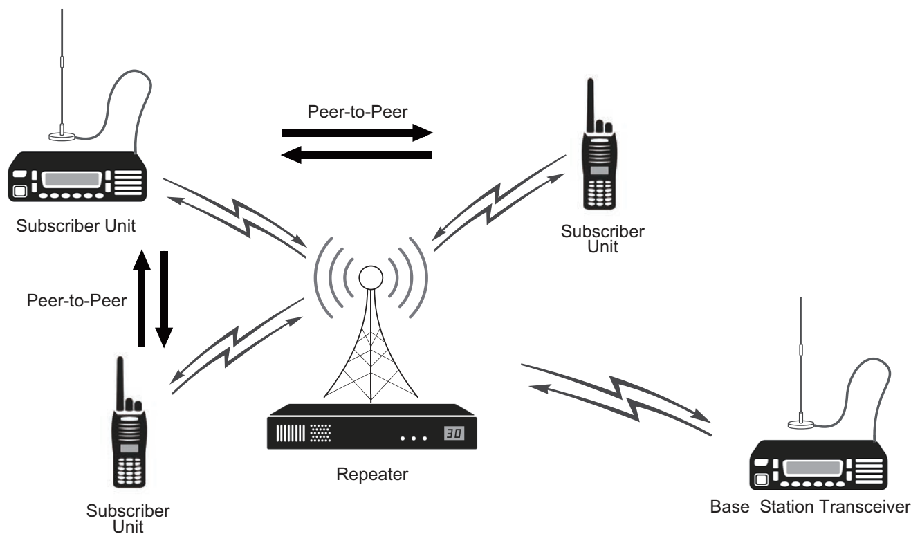
Figure 1-1 Image of Communications in a P25 Conventional System
