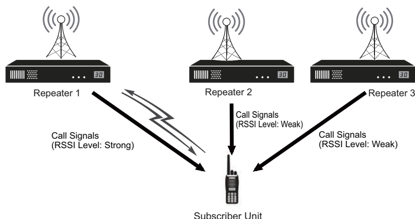
Figure 1-8 Image of Communications of P25 Voting
