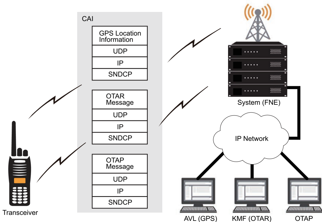
Figure 2-5 The Image of the Data Communications
