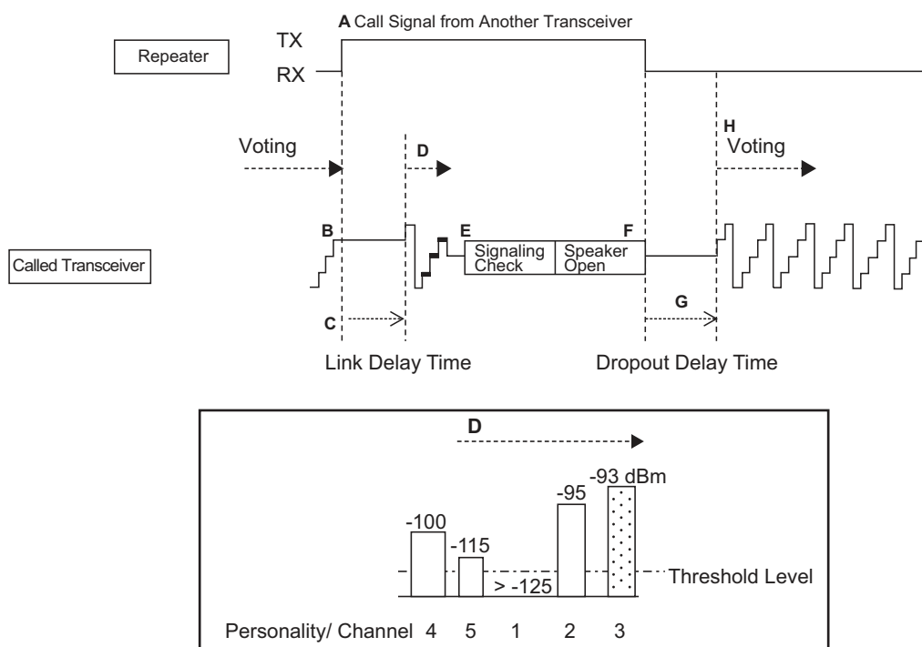
Figure 1-9 Basic Behaviors of P25 Voting
