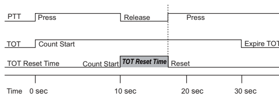
Figure 1-5 TOT Reset Time 2
