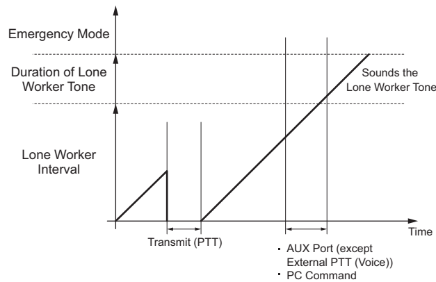
Figure 3-3 Lone Worker Mode (Mobile)
