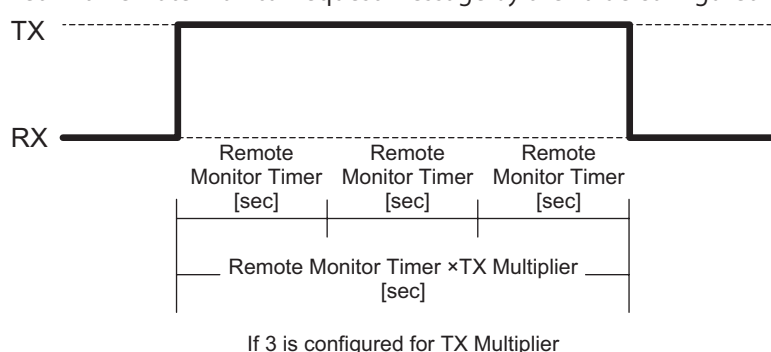
Figure 1-7 The Length of Time for Sending an Individual Call
