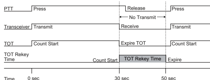
Figure 1-3 TOT Rekey Time
