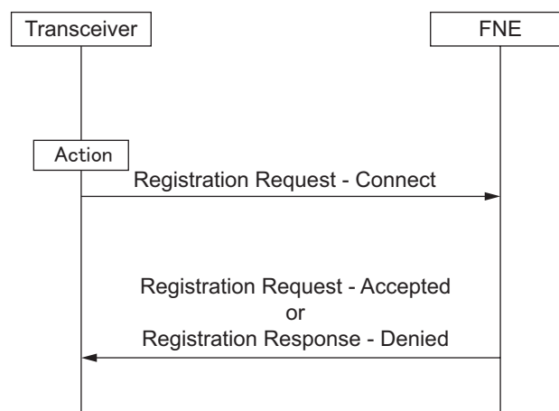
Figure 5-2 Registration Request - Connect
