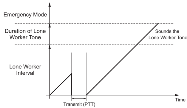
Figure 3-2 Lone Worker Mode (Portable)
