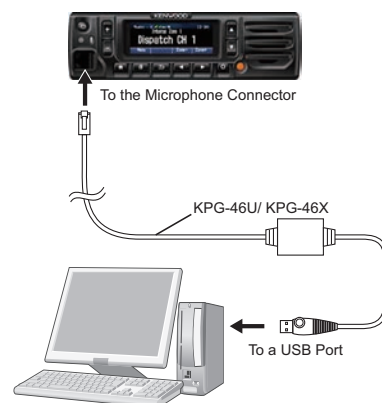
Figure 2-3 Connection of the Transceiver (Mobile) and a PC
