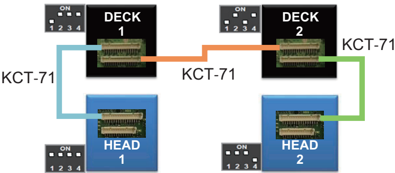
Figure 18-15 Dual Deck Dual Head Remote Mount
