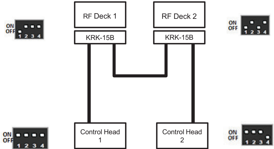
Figure 18-54 DIP Switch Configuration Dual RF Deck/ Dual Control Head
