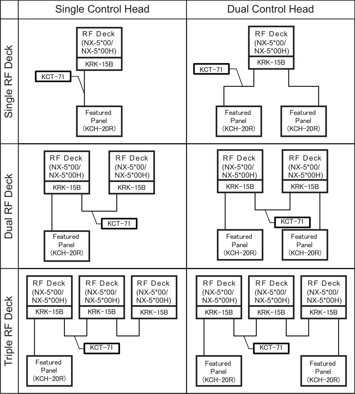
Figure 17-2 Structures of Multi RF Deck/ Multi Control Head
