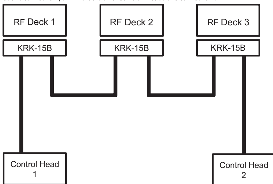
Figure 18-27 Triple RF Deck/ Dual Control Head (Power ON)
