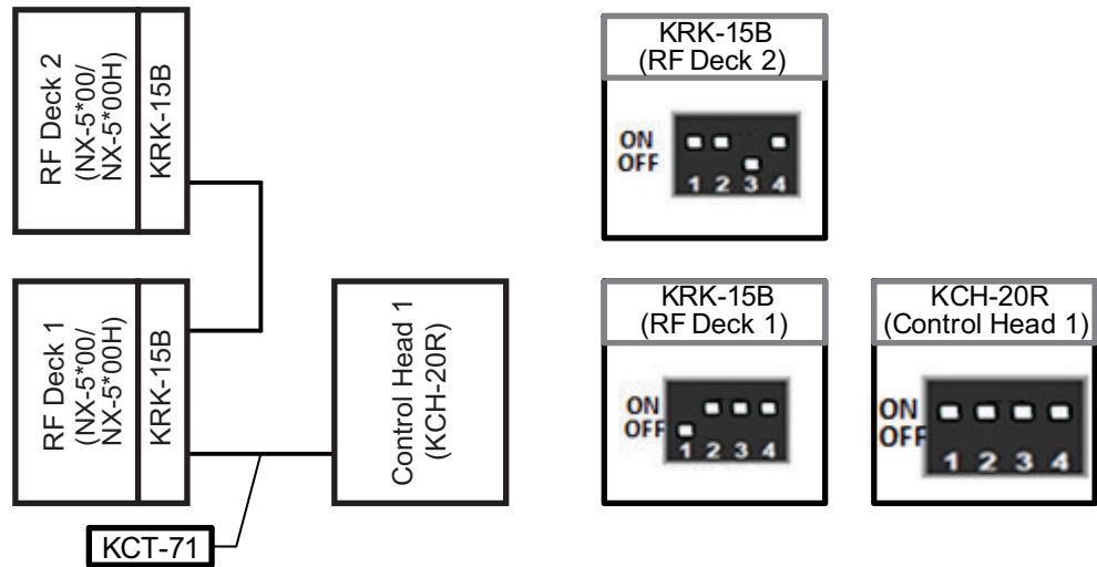
Figure 17-20 Case 3: Dual RF Deck/ Single Control Head
