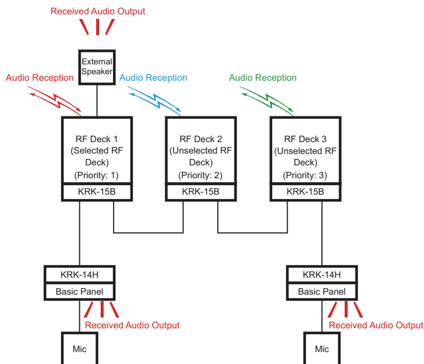
Figure 17-51 Single Audio Output (External Speaker = Internal + External)
