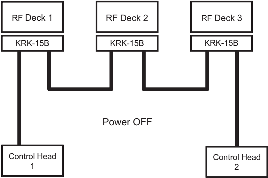
Figure 18-32 Triple RF Deck/ Dual Control Head (Power OFF)
