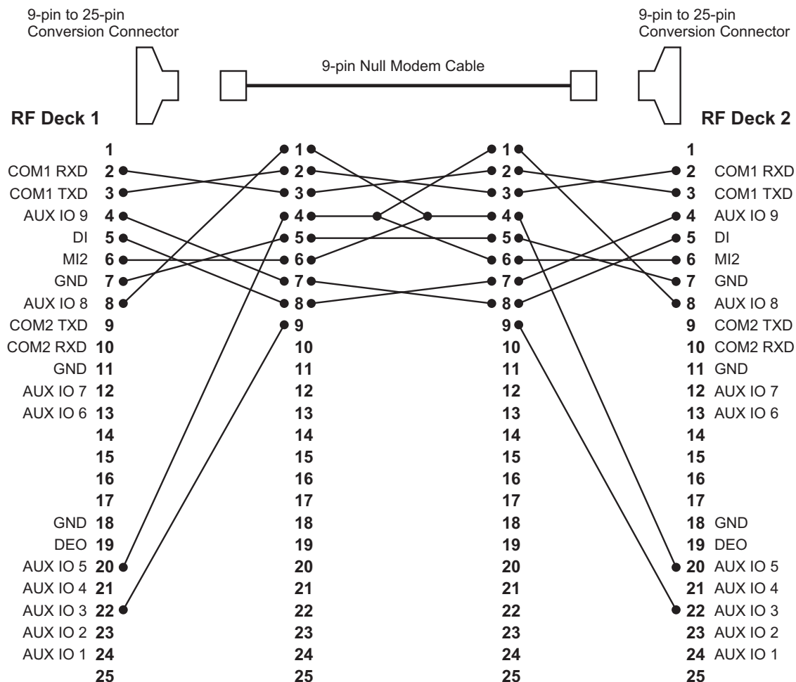
Figure 17-91 Wiring Diagram (COM port 1)
