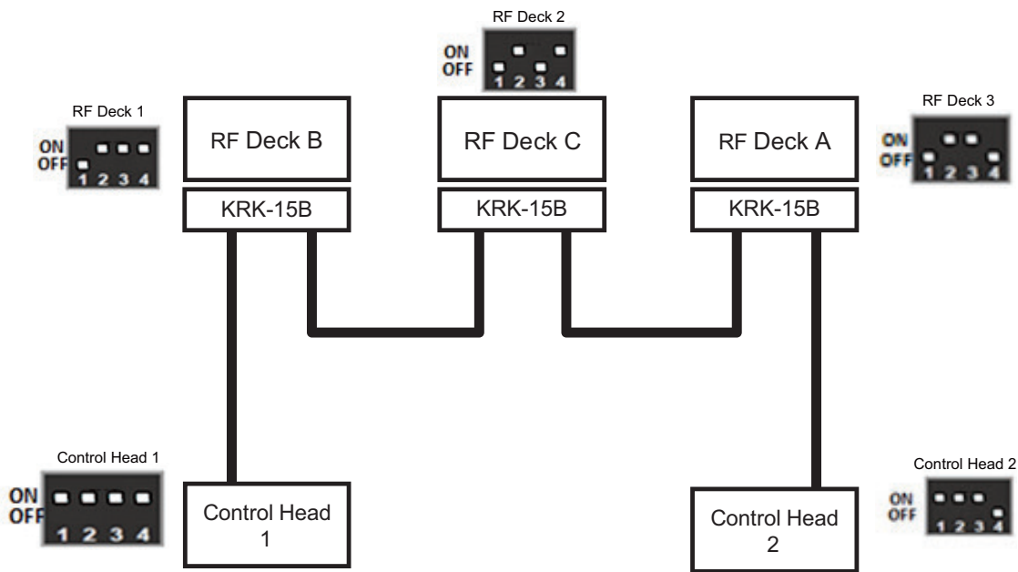
Figure 18-73 DIP Switch Configuration
