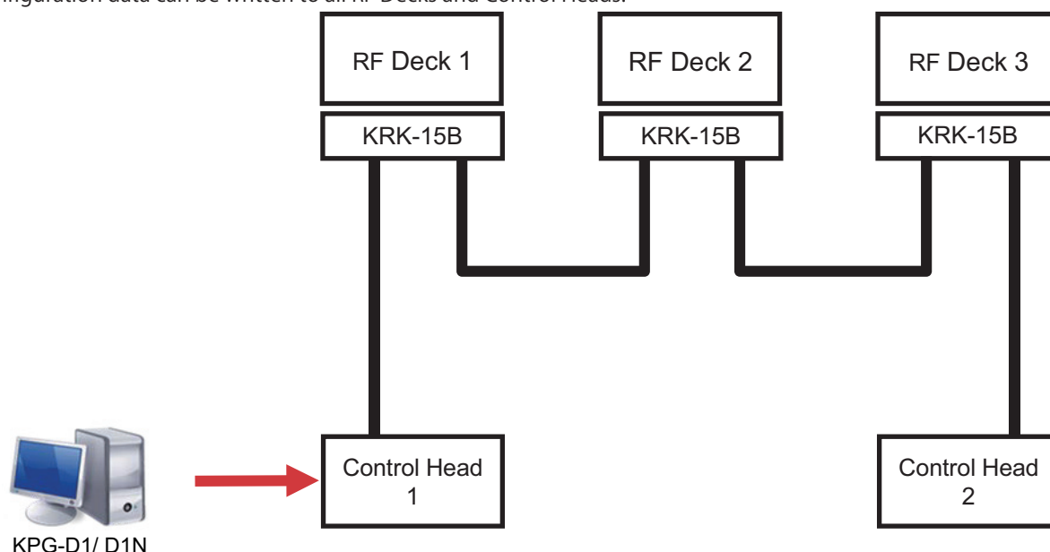
Figure 18-65 Triple RF Deck/ Dual Control Head (FPU Setting)
