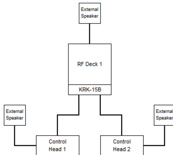
Figure 3-1 Diagram of the Single RF Deck/ Dual Control Head Structure
