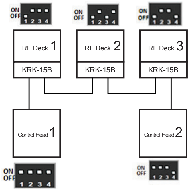
Figure 17-15 DIP Switch Configuration
