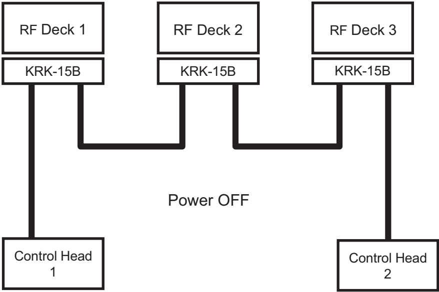
Figure 18-51 Triple RF Deck/ Dual Control Head (Power OFF)
