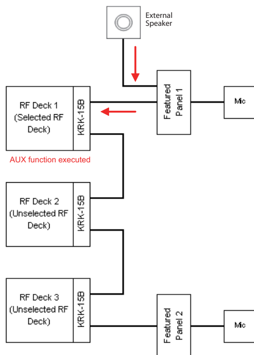
Figure 17-60 Example of When the AUX Input Is Configured for Control Heads
