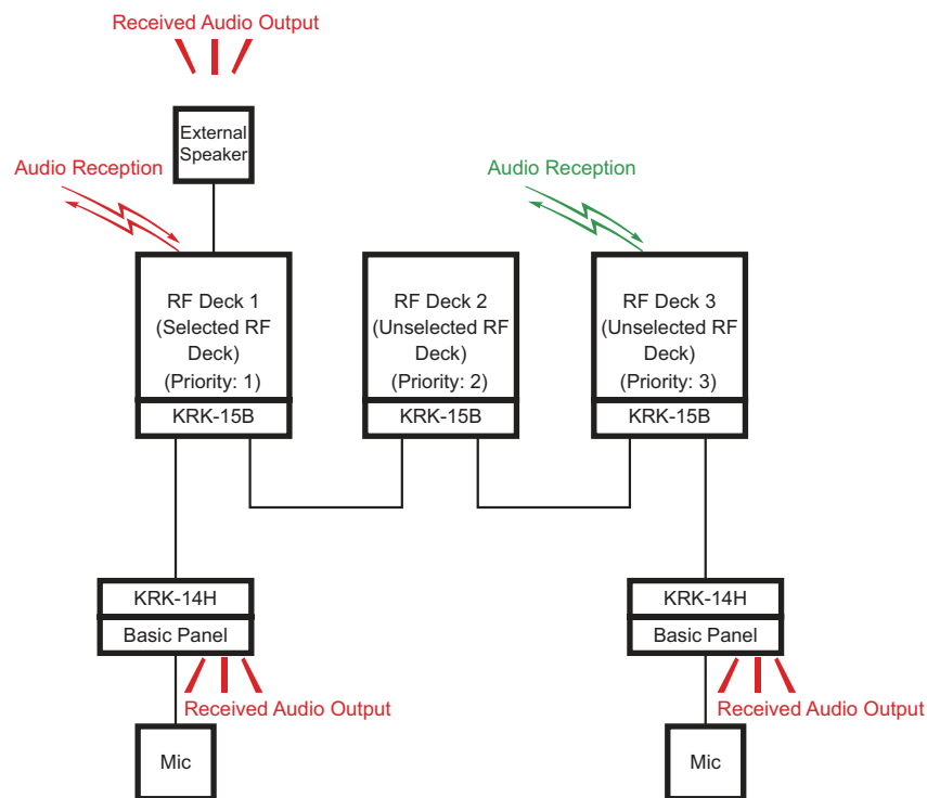
Figure 17-54 Single Audio Output 2
