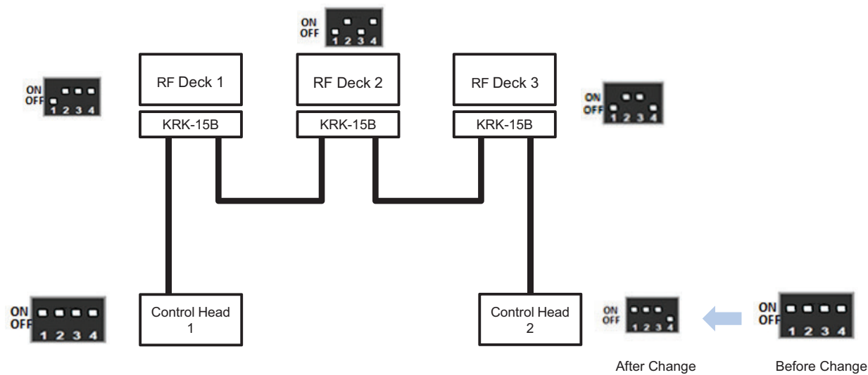
Figure 18-35 DIP Switch Configuration Triple RF Deck/ Dual Control Head
