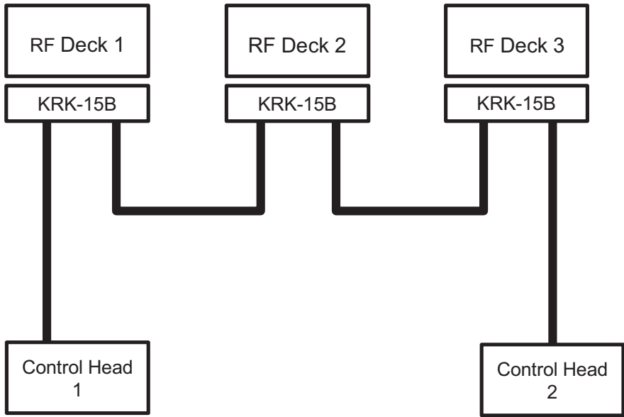
Figure 18-21 Triple RF Deck/ Dual Control Head (Power ON)
