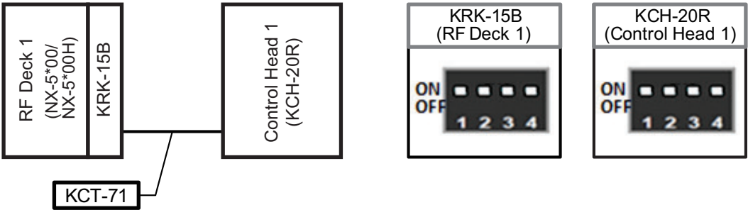
Figure 17-18 Case 1: Single RF Deck/ Single Control Head
