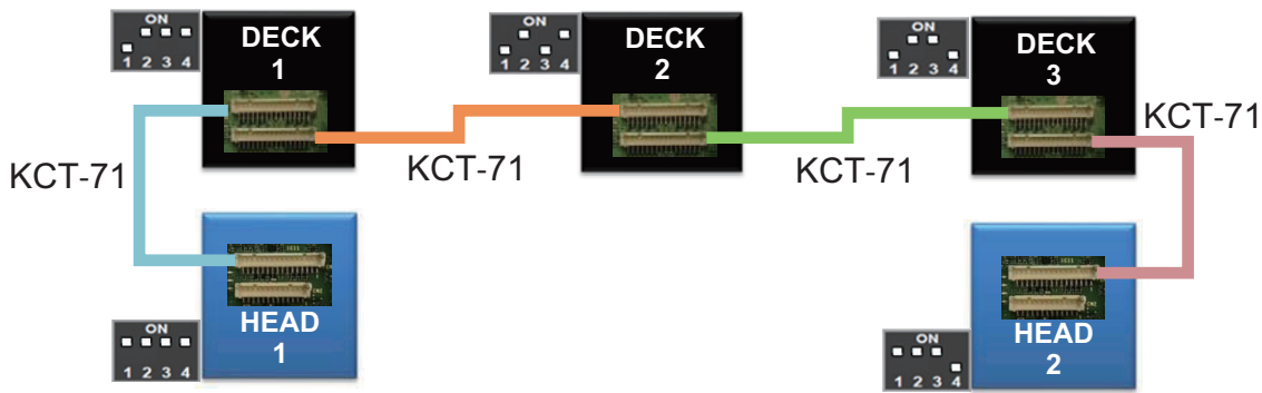
Figure 18-17 Triple Deck Dual Head Remote Mount
