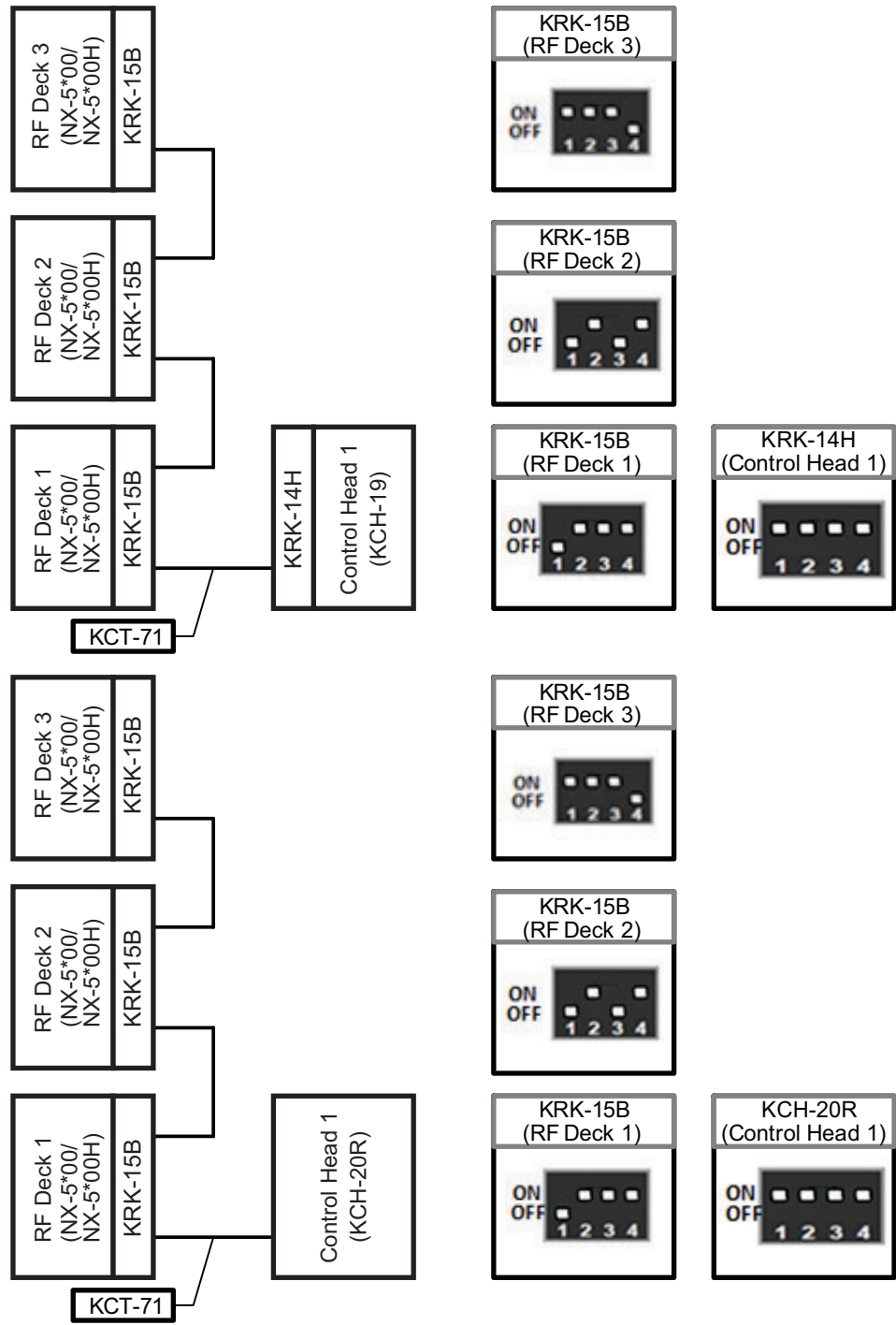
Figure 17-22 Case 5: Triple RF Deck/ Single Control Head
