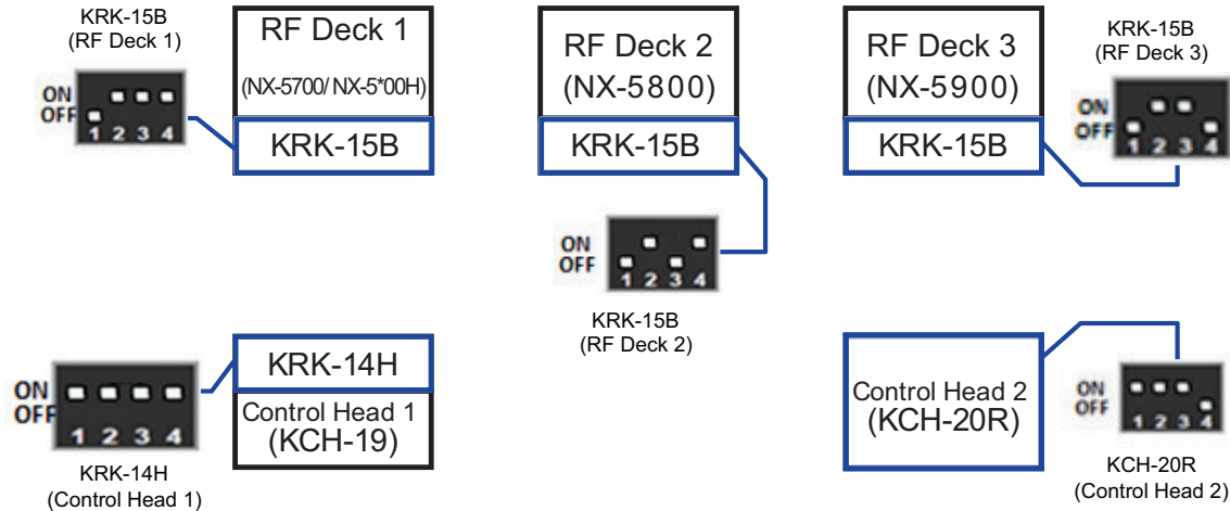
Figure 17-12 DIP Switch Configuration
