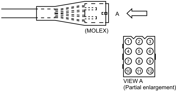
Figure 18-91 KCT-72 (Connection Cable)
