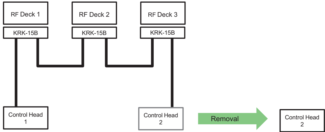
Figure 18-33 Removal of Control Head 2
