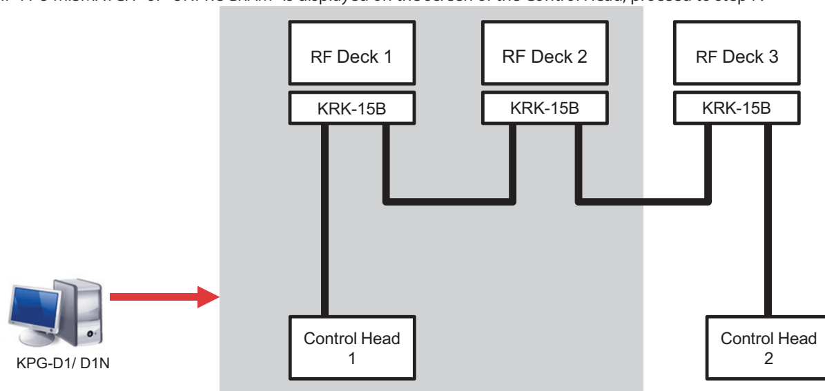
Figure 18-28 Triple RF Deck/ Dual Control Head (FPU Setting 1)
