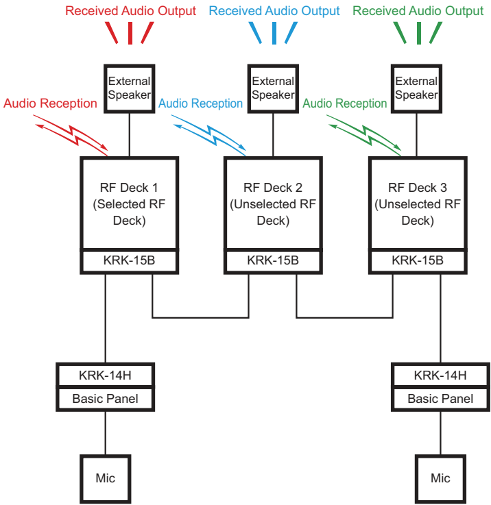
Figure 17-50 Multi Audio Output (External Speaker = On)
