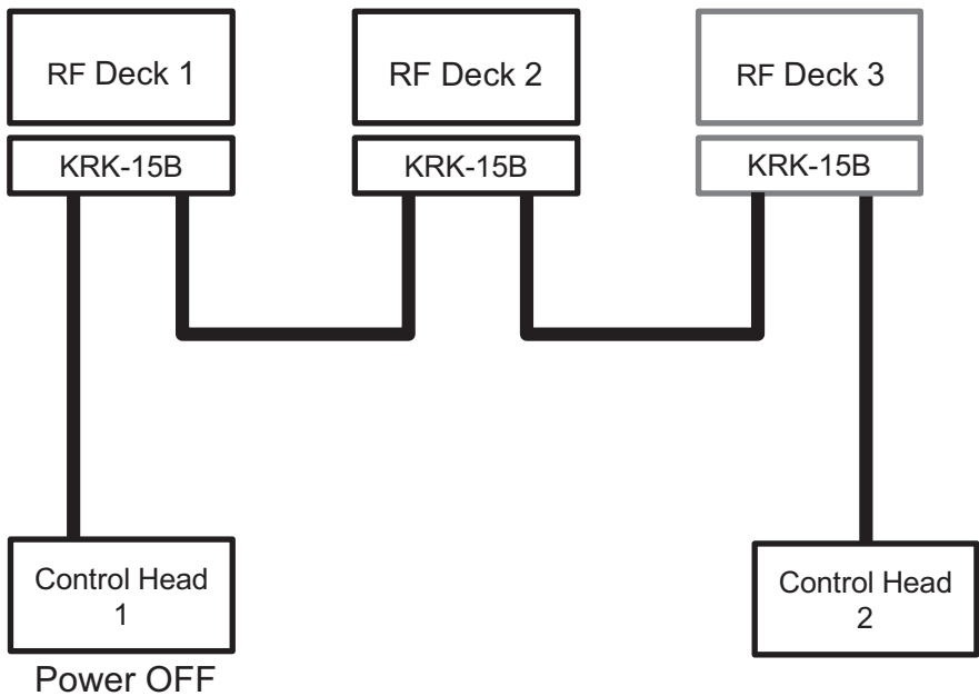
Figure 18-59 Triple RF Deck/ Dual Control Head (Power OFF)
