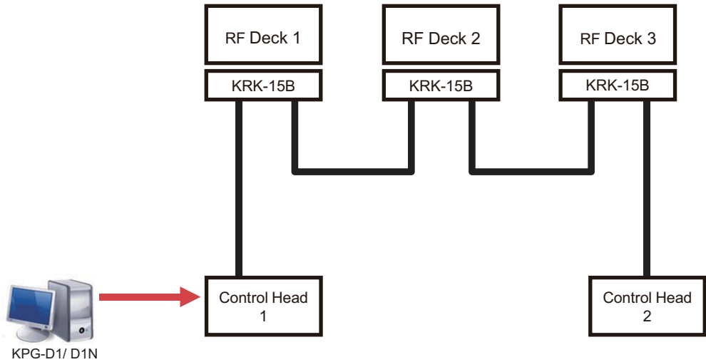
Figure 17-89 Triple RF Deck/ Dual Control Head (FPU Setting)
