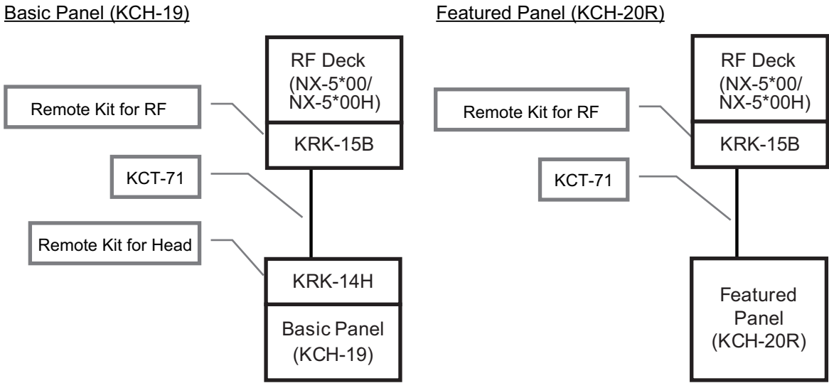
Figure 17-3 Single RF Deck/ Single Control Head
