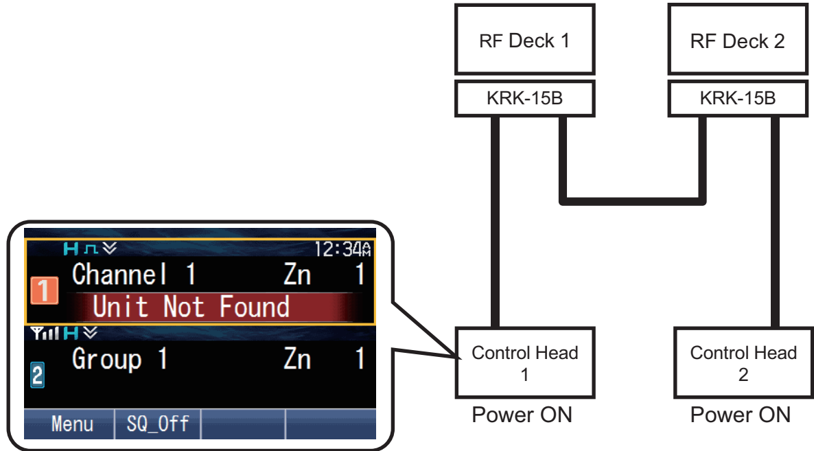
Figure 18-55 Dual RF Deck/ Dual Control Head (Power ON)
