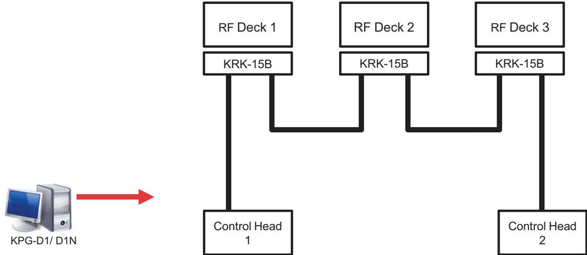
Figure 18-45 Triple RF Deck/ Dual Control Head (FPU Setting)
