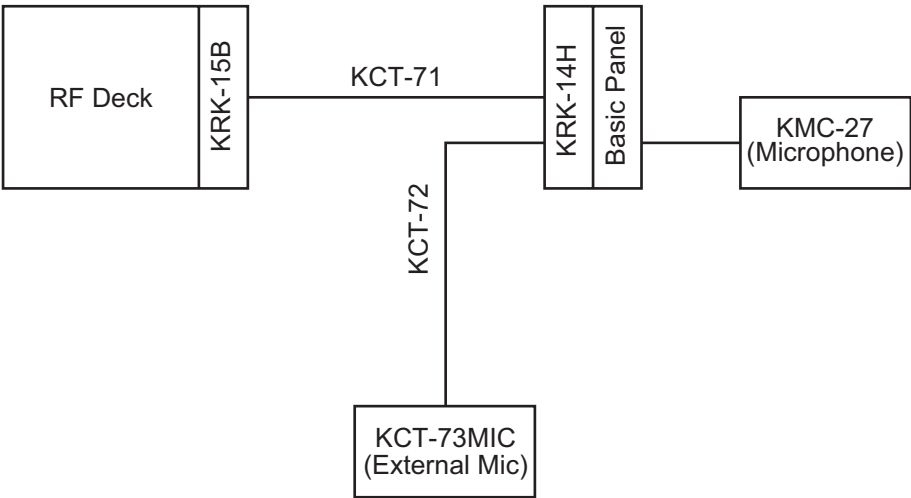
Figure 12-4 Control Head Mic Input
