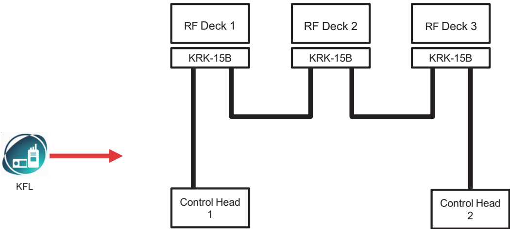
Figure 18-30 Triple RF Deck/ Dual Control Head (Firmware Setting)
