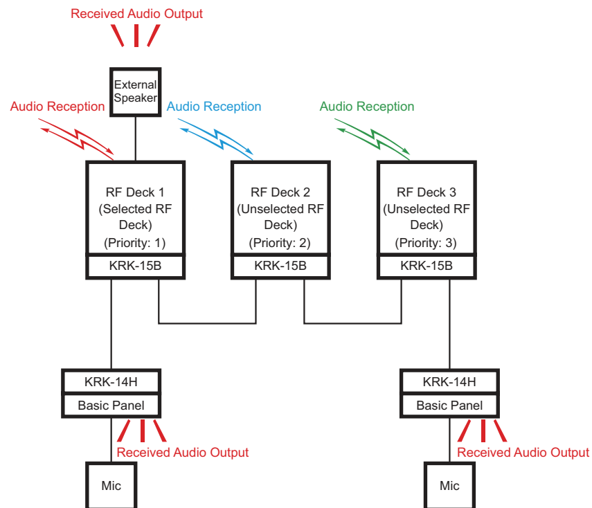
Figure 17-55 Single Audio Output 3
