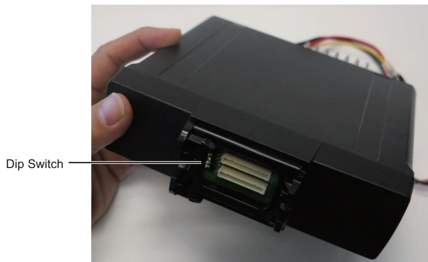
Figure 18-4 Attachment of KRK-15BM
