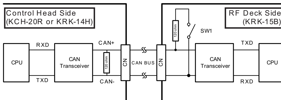
Figure 17-16 Block Diagram of CAN Communication
