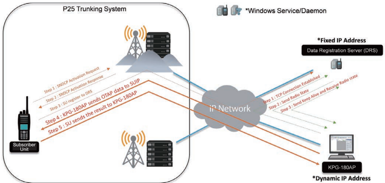
Figure 2-8 Example of the P25 Trunking OTAP Structure
