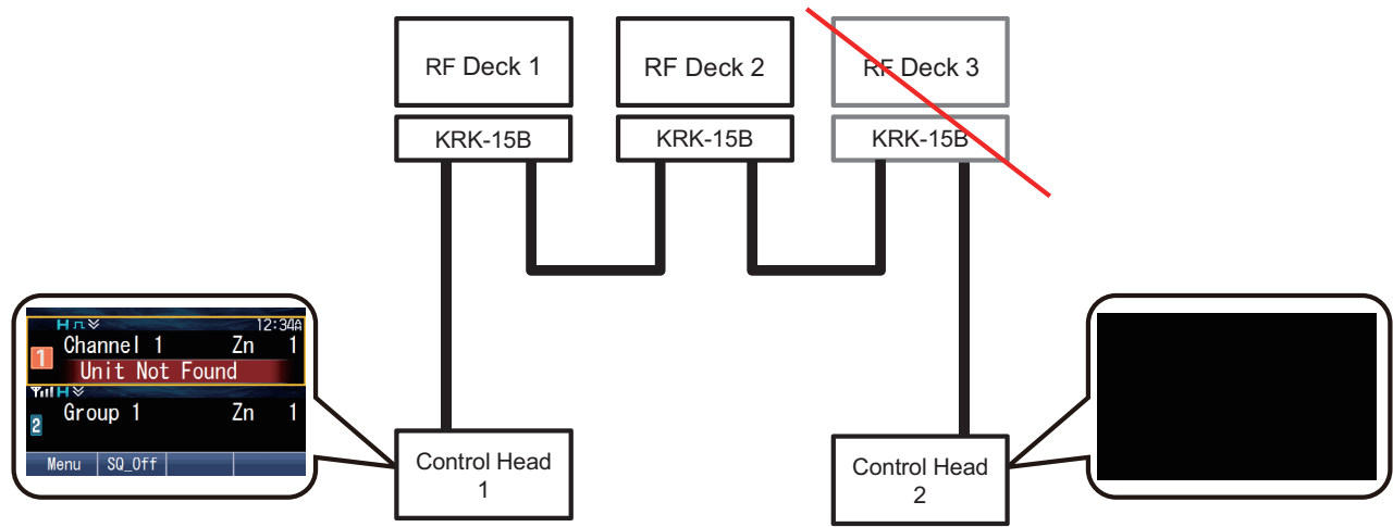
Figure 18-58 Breakdown of RF Deck 3
