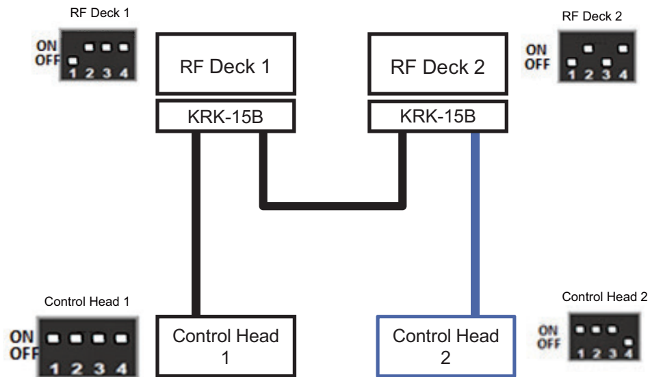
Figure 18-62 Dual RF Deck/ Dual Control Head
