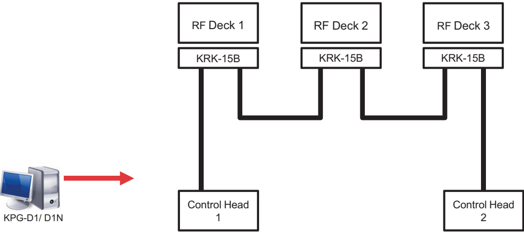
Figure 18-38 Triple RF Deck/ Dual Control Head (FPU Setting)
