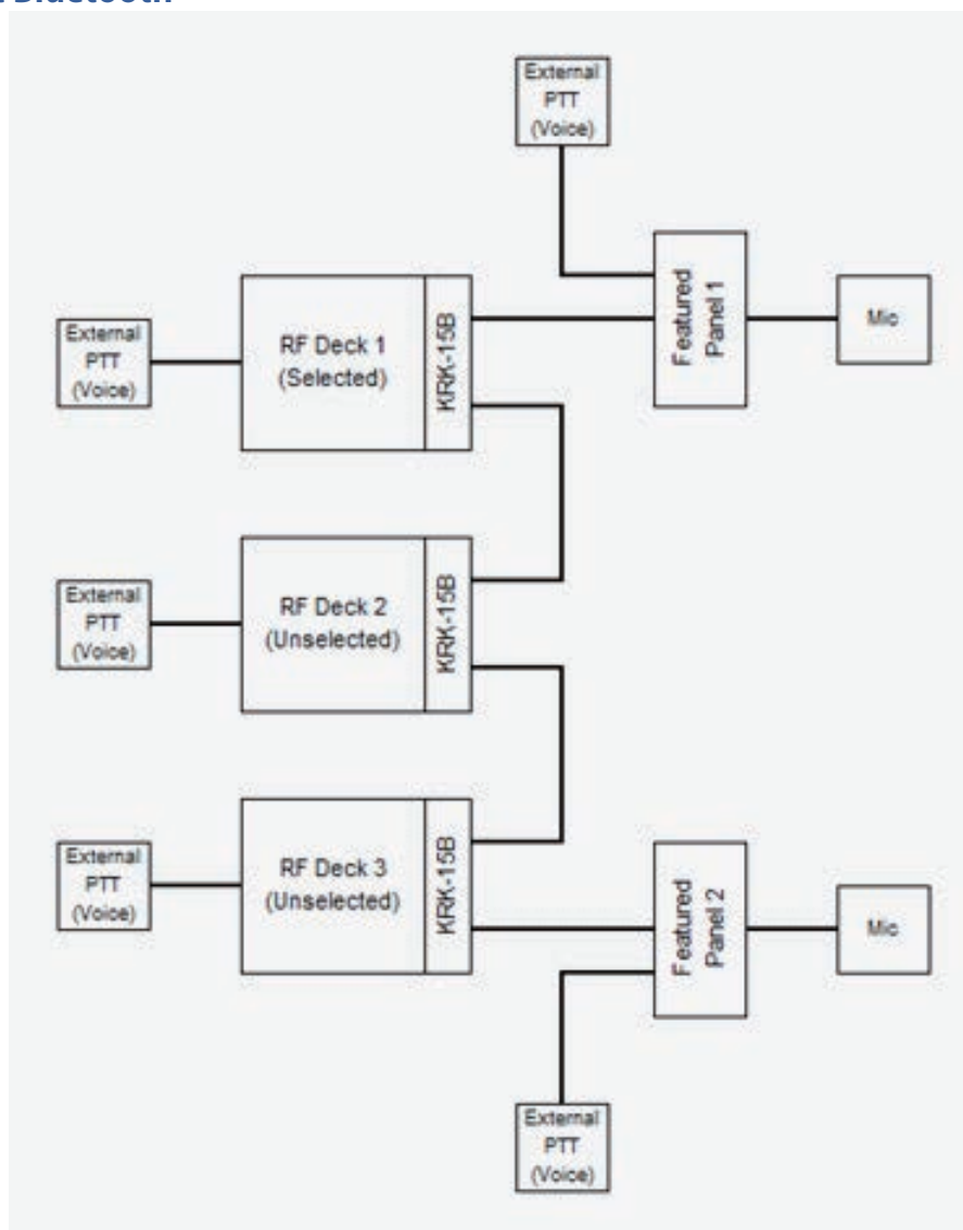
Figure 17-35 Case 1: Without Bluetooth
