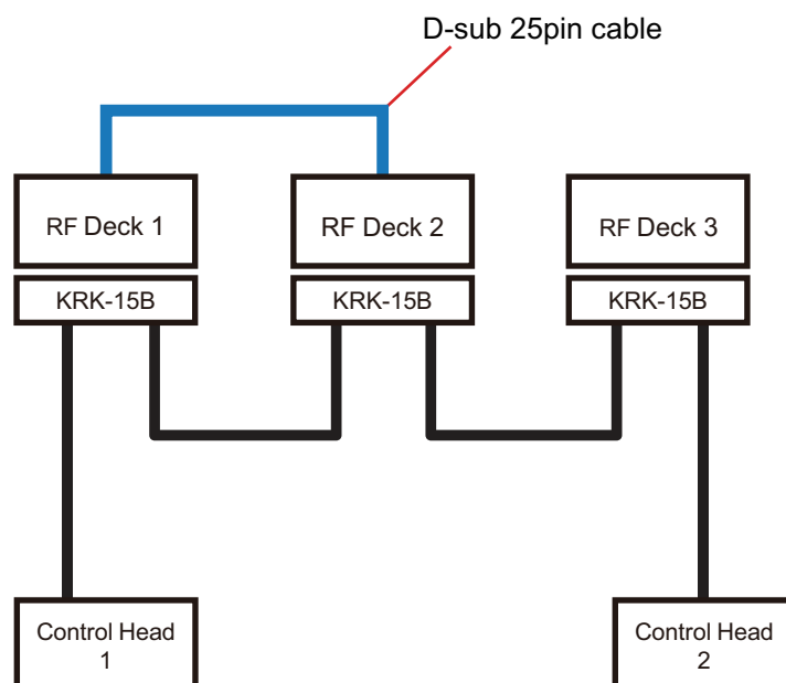
Figure 17-90 Connection Diagram
