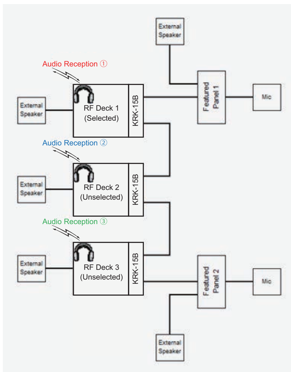
Figure 17-75 Pattern of Emitting Audio (RF Deck)
