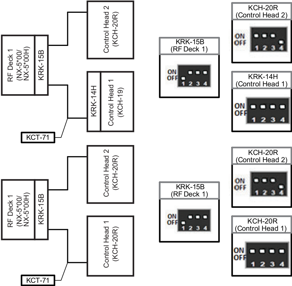
Figure 17-19 Case 2: Single RF Deck/ Dual Control Head
