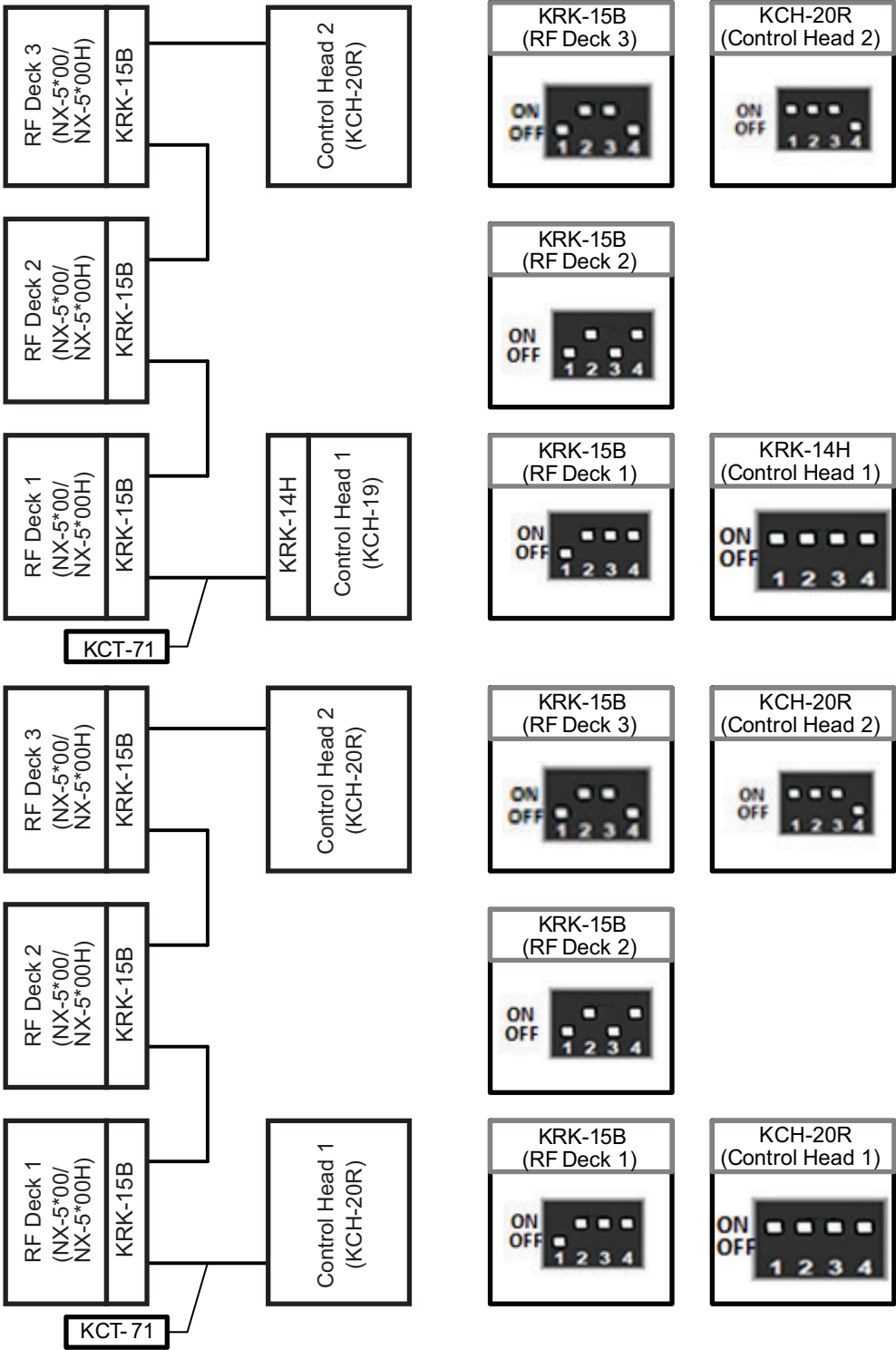
Figure 17-23 Case 6: Triple RF Deck/ Dual Control Head
