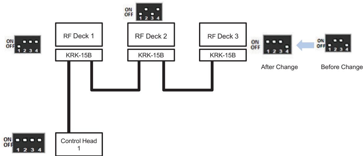
Figure 18-48 DIP Switch Configuration Triple RF Deck/ Single Control Head
