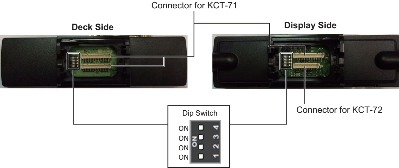
Figure 18-11 Connector Arrangement and Cable Connection
