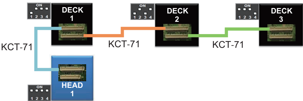
Figure 18-16 Triple Deck Single Head Remote Mount
