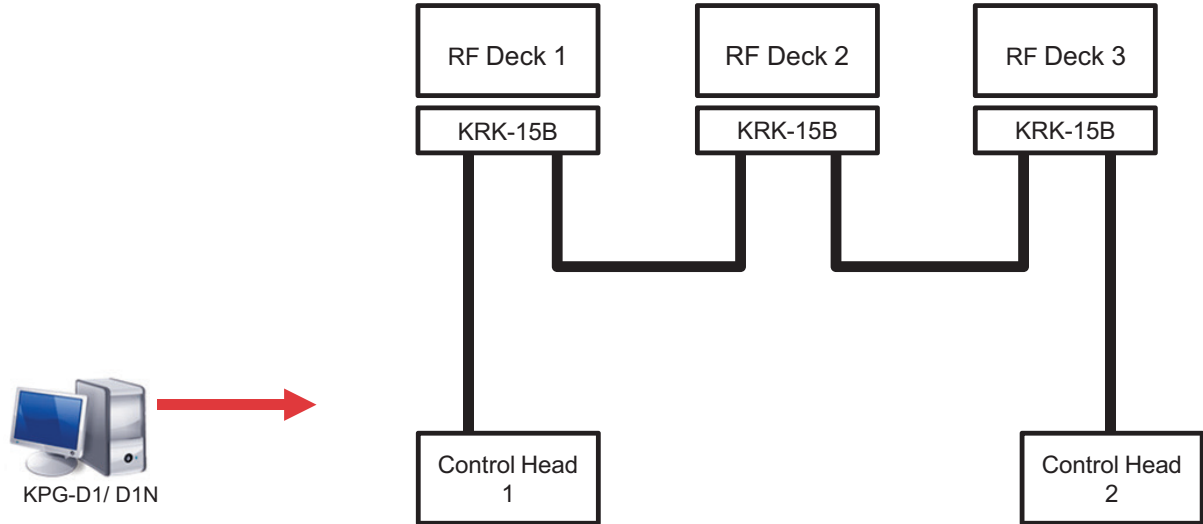
Figure 18-23 Triple RF Deck/ Dual Control Head (FPU Setting)
