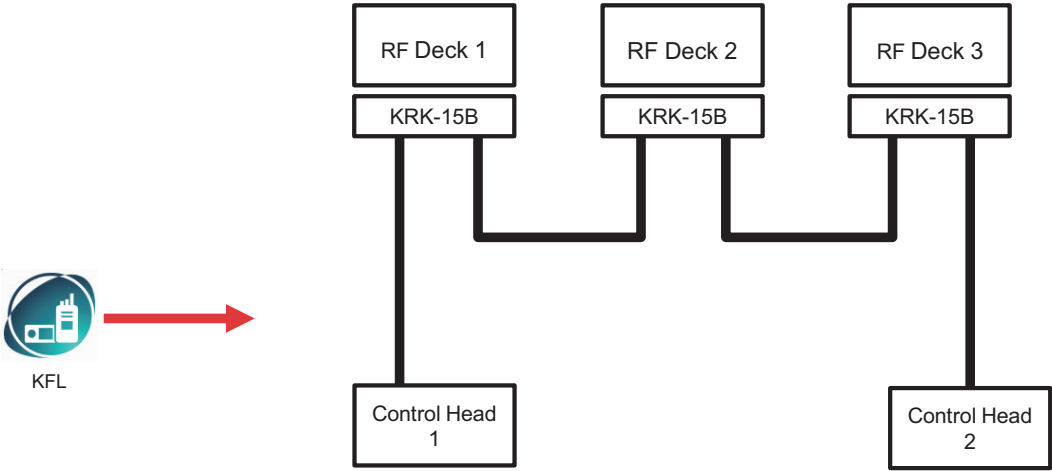
Figure 18-37 Triple RF Deck/ Dual Control Head (Firmware Setting)
