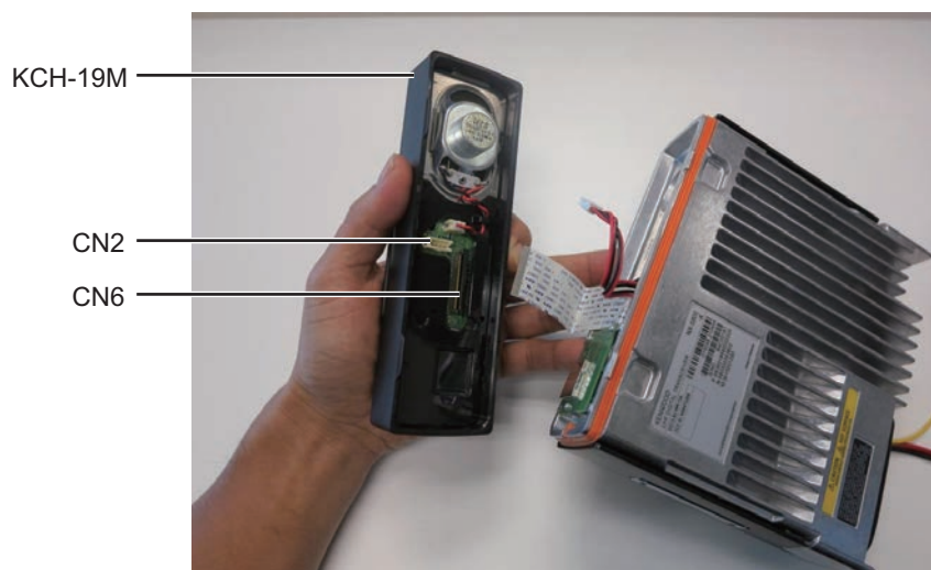
Figure 18-2 Removal of the Cables
