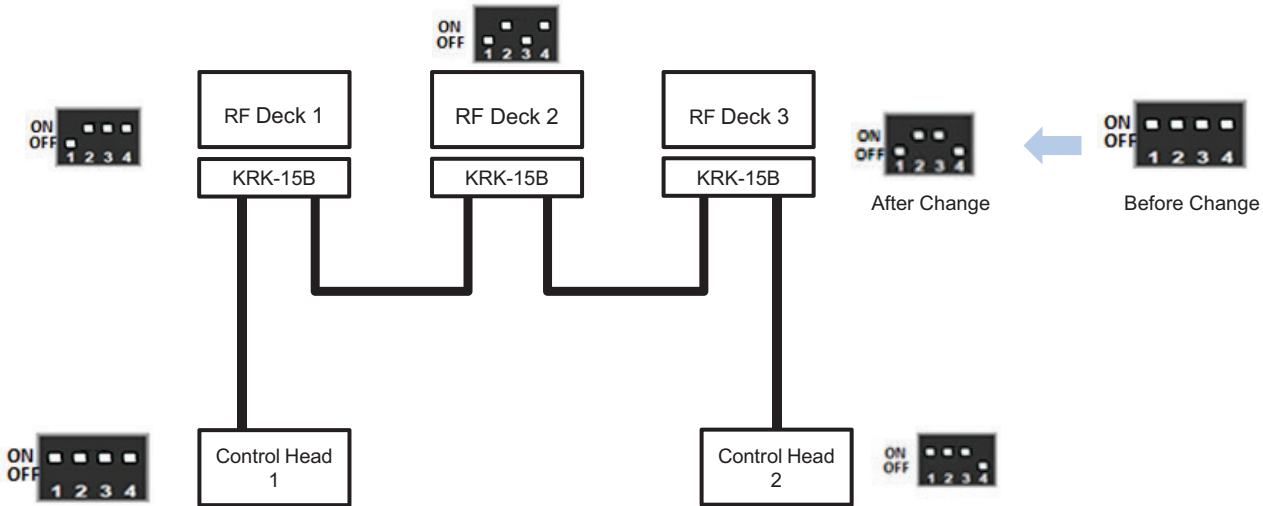
Figure 18-26 DIP Switch Configuration Triple RF Deck/ Dual Control Head
