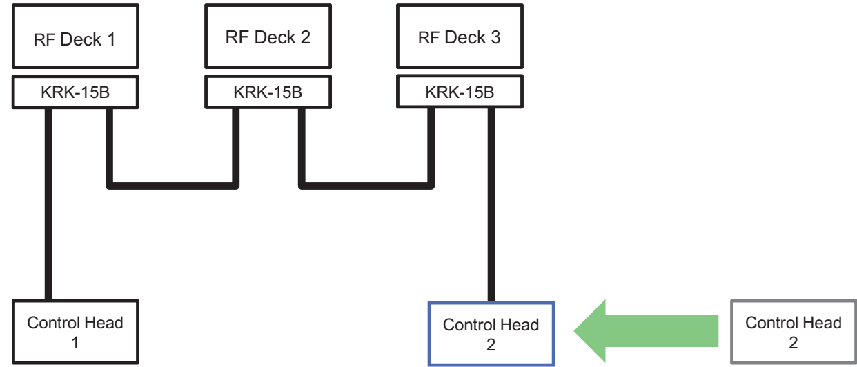
Figure 18-19 Installation of Control Head 2
