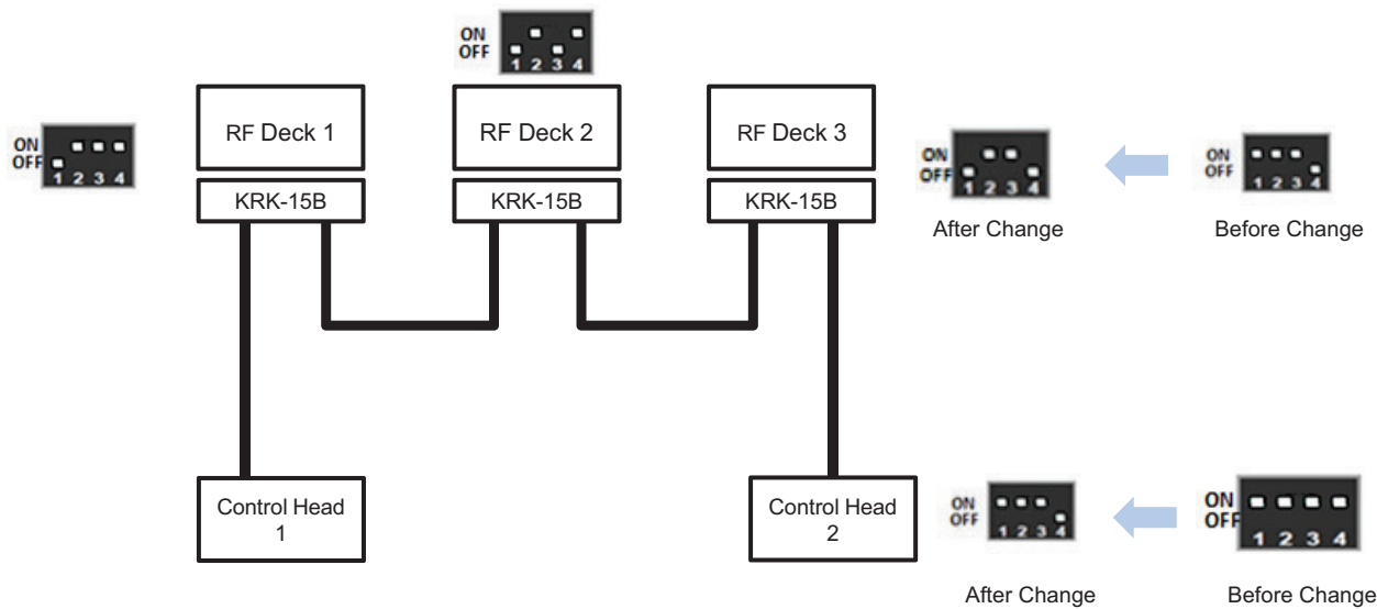
Figure 18-20 DIP Switch Configuration Triple RF Deck/ Dual Control Head
