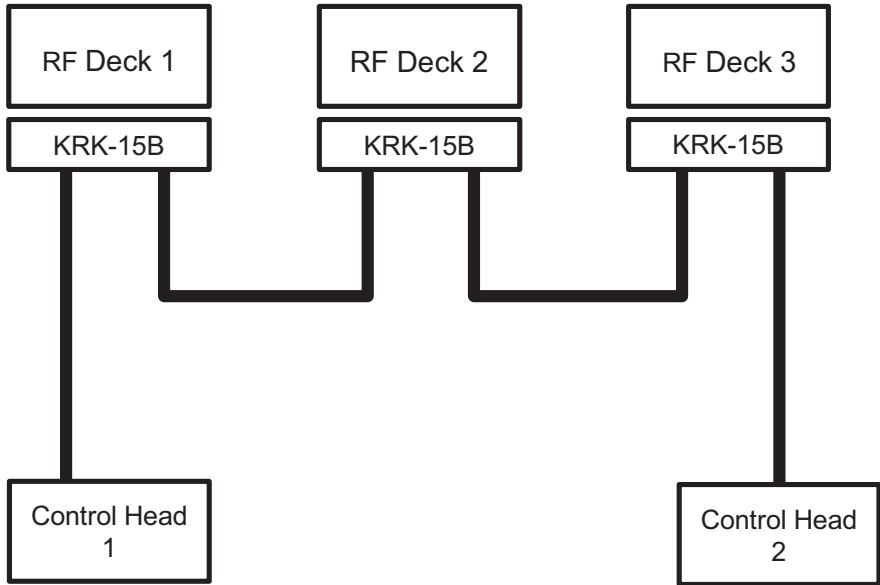
Figure 18-36 Triple RF Deck/ Dual Control Head (Power ON)
