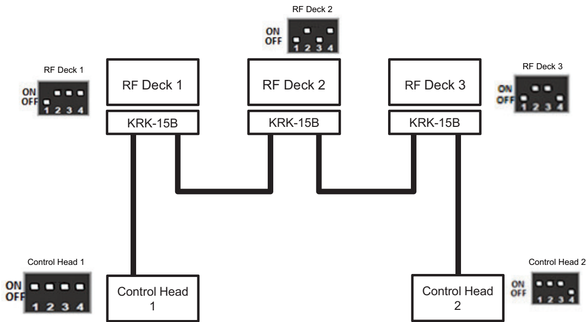
Figure 18-64 DIP Switch Configuration
