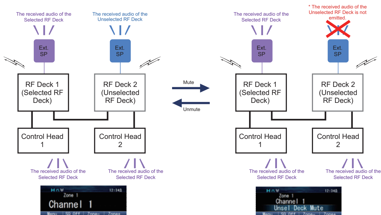
Figure 17-40 Unselected RF Deck Speaker
