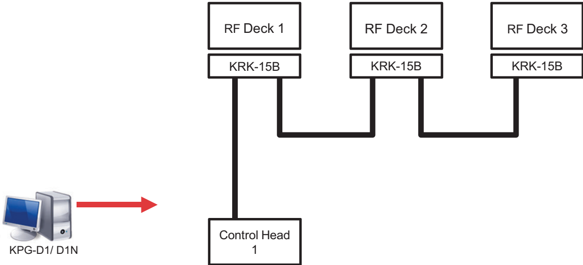
Figure 18-50 Triple RF Deck/ Single Control Head (FPU Setting)
