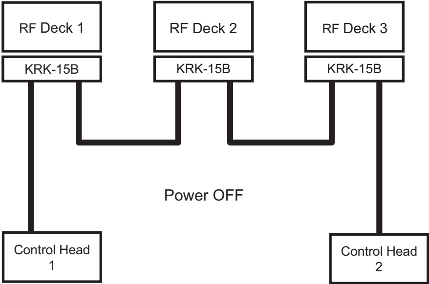
Figure 18-46 Triple RF Deck/ Dual Control Head (Power OFF)
