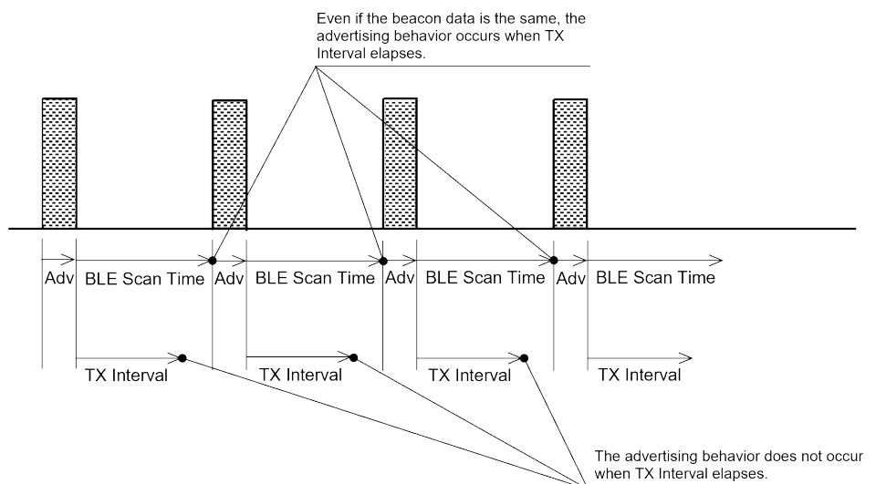
Figure 10-6 Relationship of TX Interval and BLE Scan Time (If the BLE Scan Time Configuration Is Longer Than the TX Interval Configuration)
