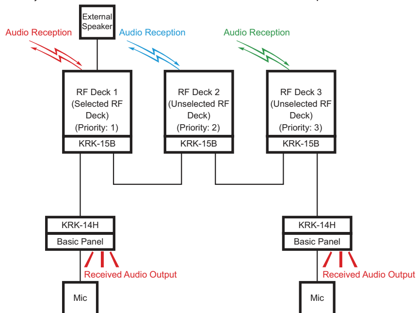
Figure 17-47 Single Audio Output (External Speaker = Off)
