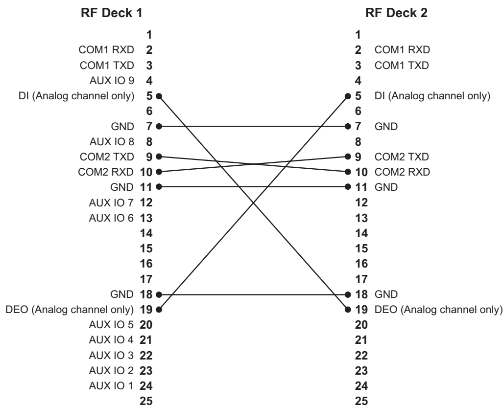
Figure 17-92 Wiring Diagram (COM port 2)
