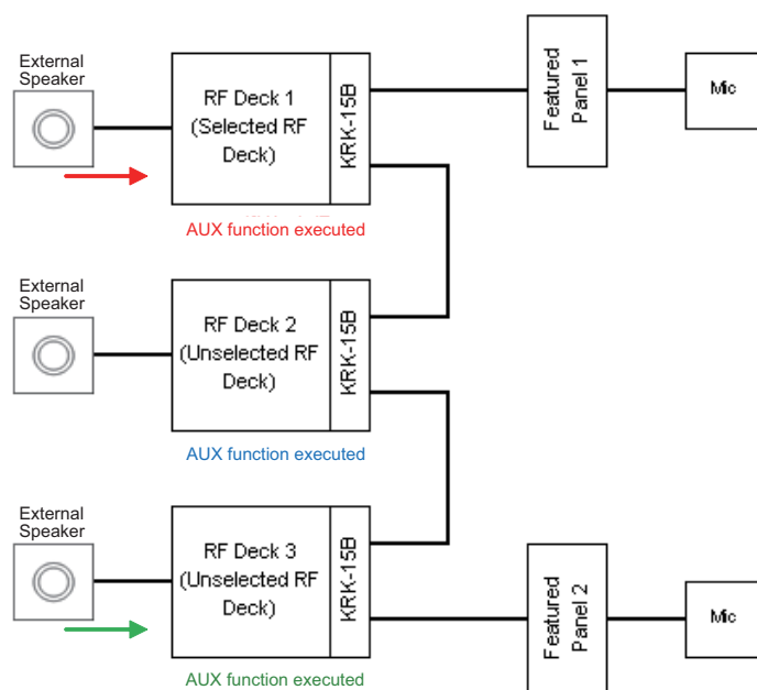
Figure 17-59 Example of When the AUX Input Is Configured for RF Decks
