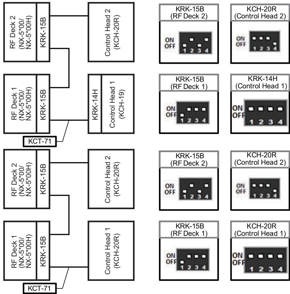
Figure 17-21 Case 4: Dual RF Deck/ Dual Control Head
