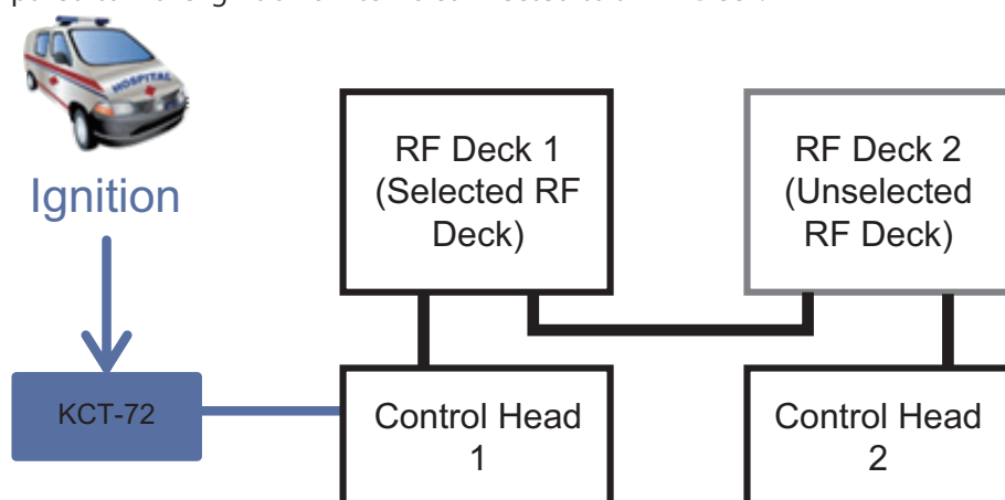
Figure 17-61 Example of When the Ignition of a Control Head Is Used
