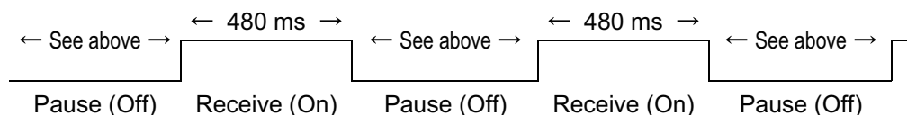
Figure 7-2 Battery Saver (DMR Tier III Trunking)
