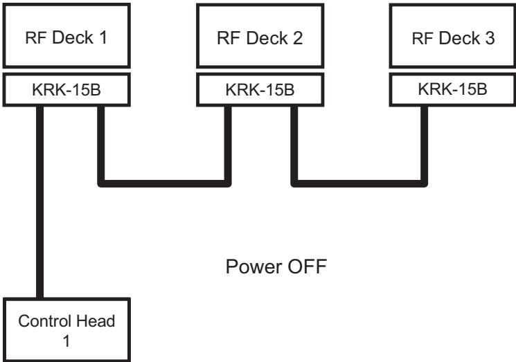
Figure 18-18 Triple RF Deck/ Single Control Head (Power OFF)
