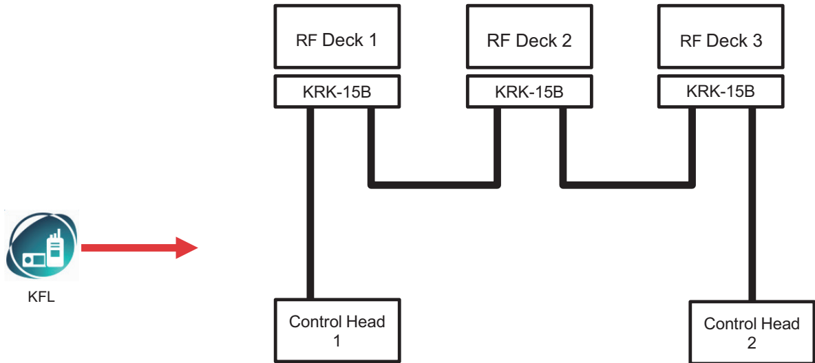
Figure 18-44 Triple RF Deck/ Dual Control Head (Firmware Setting)
