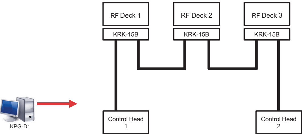
Figure 18-31 Triple RF Deck/ Dual Control Head (FPU Setting 2)
