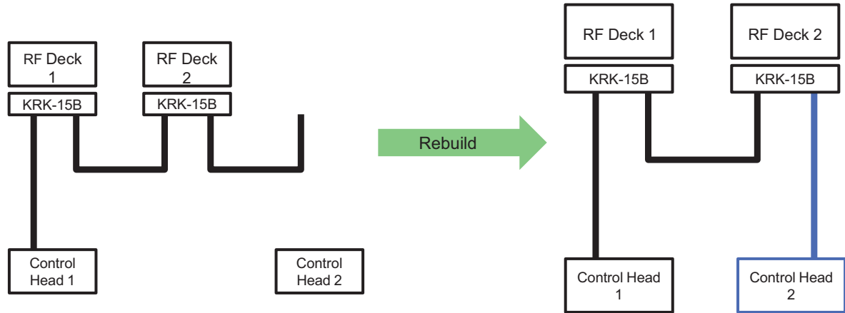
Figure 18-53 Dual RF Deck/ Dual Control Head
