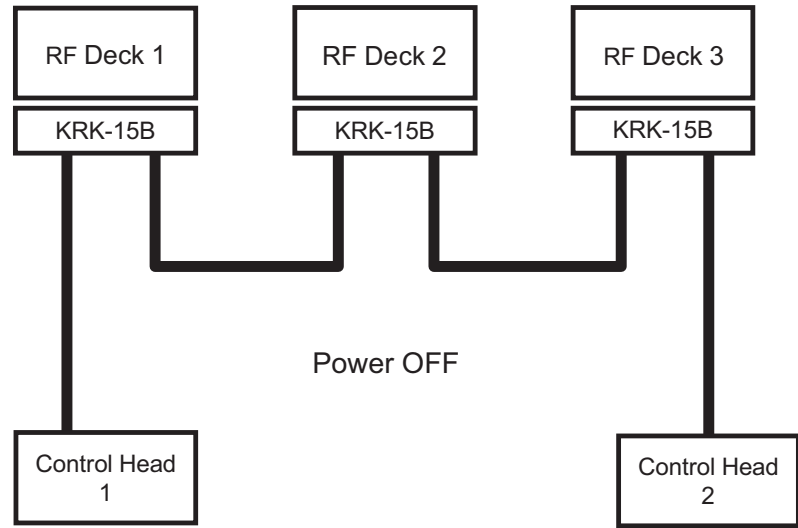
Figure 18-39 Triple RF Deck/ Dual Control Head (Power OFF)
