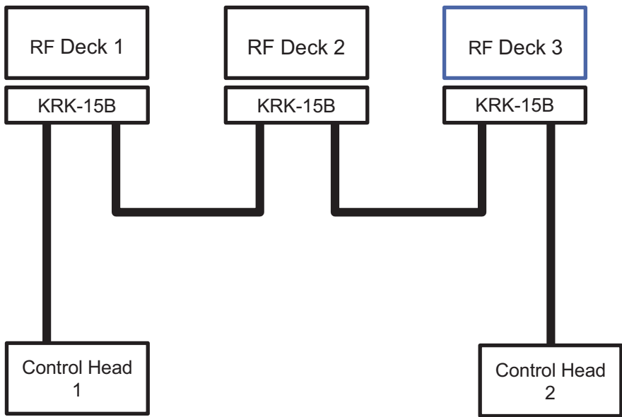
Figure 18-63 Triple RF Deck/ Dual Control Head
