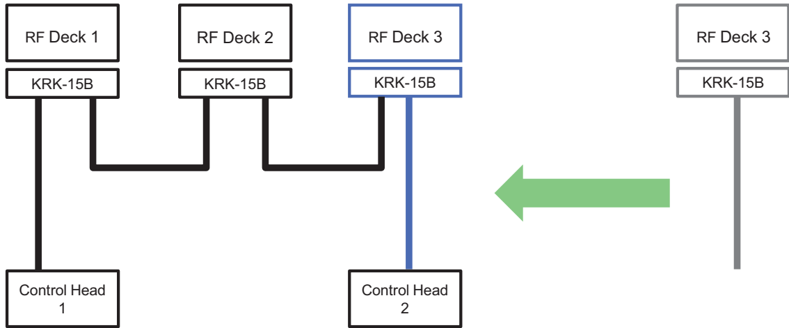
Figure 18-25 Installation of RF Deck 3/ KCT-71
