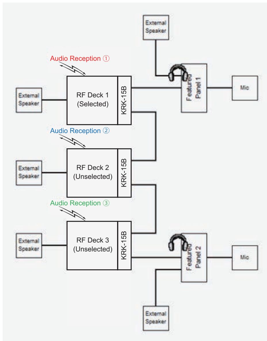
Figure 17-76 Pattern of Emitting Audio (Control Head)
