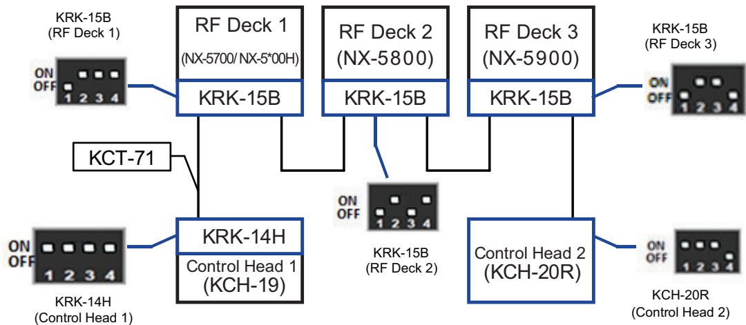
Figure 17-13 Connection of RF Decks and Control Heads
