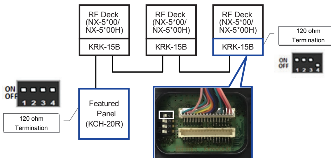
Figure 17-17 Triple RF Deck/ Single Control Head
