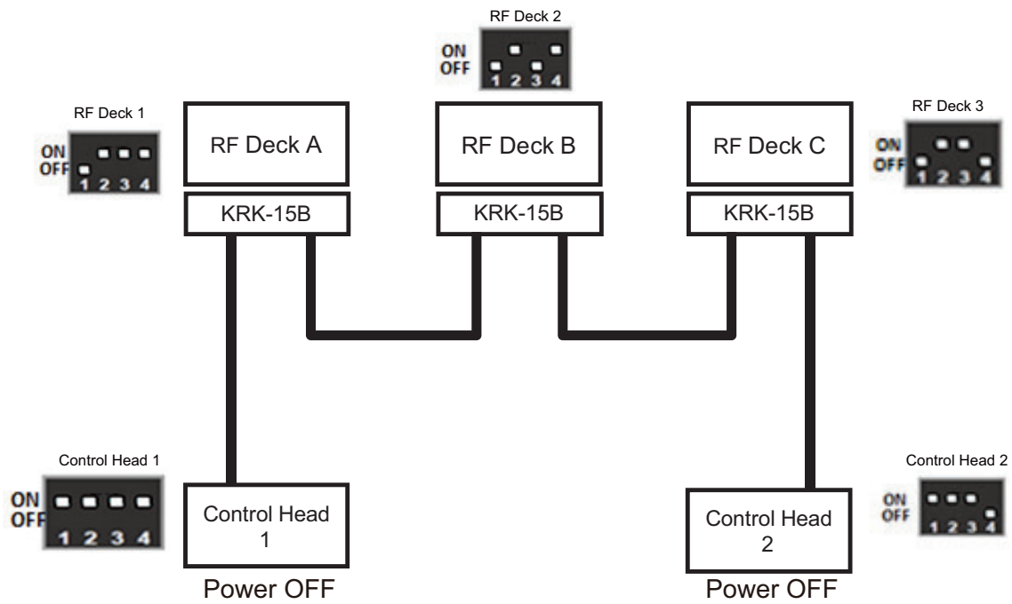
Figure 18-71 Triple RF Deck/ Dual Control Head (Power OFF)
