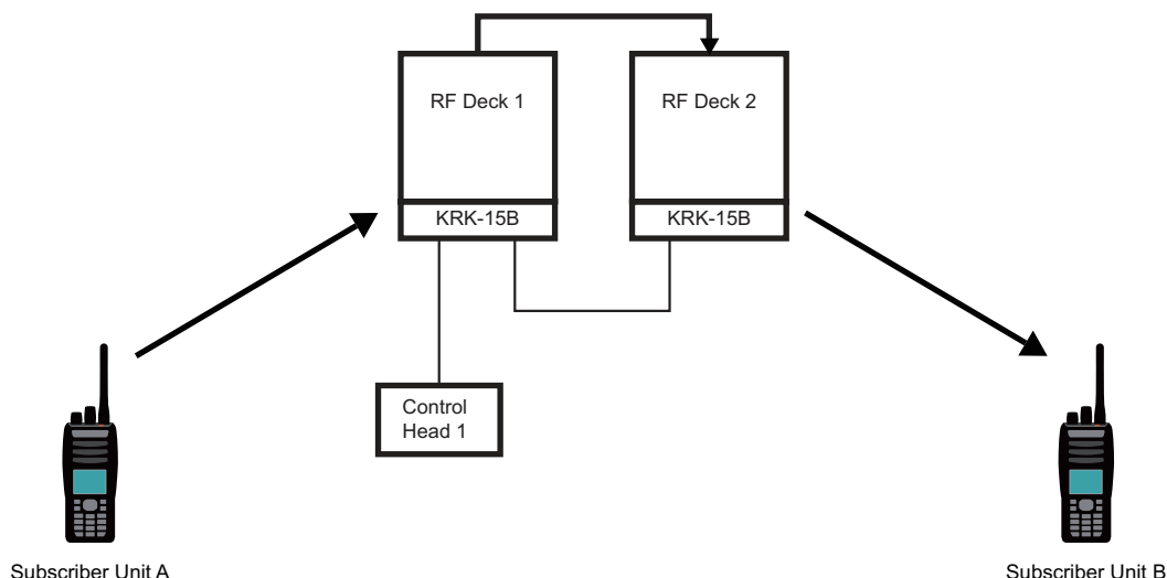
Figure 17-84 Outline of Mobile Relay Station
