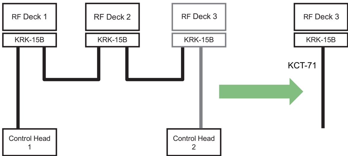
Figure 18-60 Removal of RF Deck 3/ KCT-71
