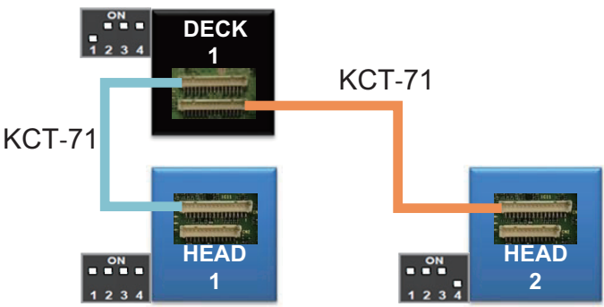
Figure 18-13 Single Deck Dual Head Remote Mount
