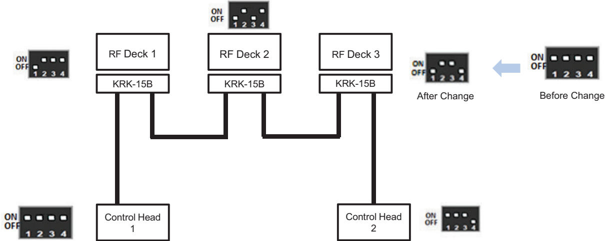
Figure 18-42 DIP Switch Configuration Triple RF Deck/ Dual Control Head
