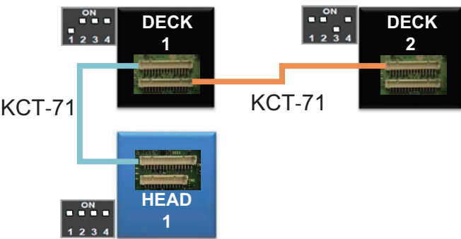
Figure 18-14 Dual Deck Single Head Remote Mount
