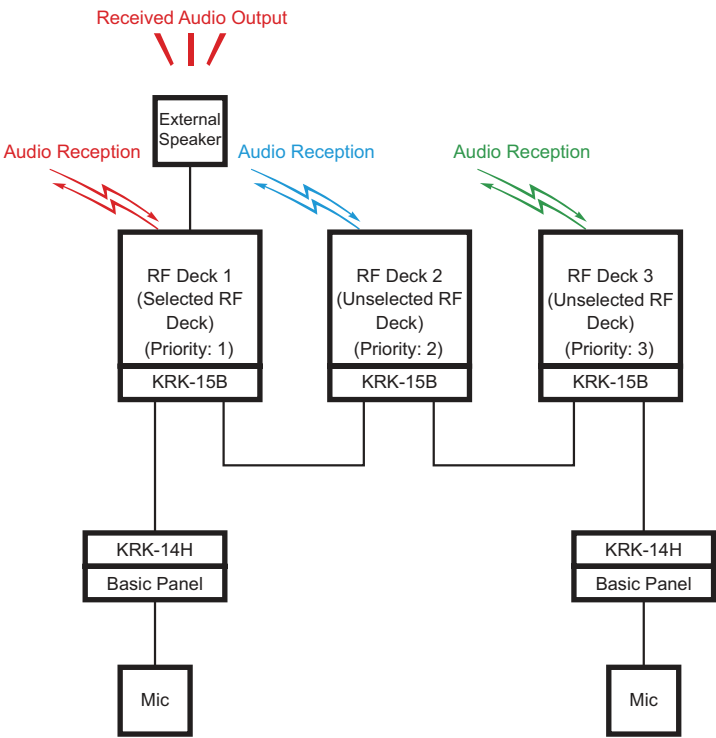
Figure 17-49 Single Audio Output (External Speaker = On)
