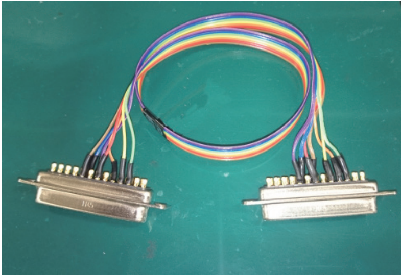
Figure 17-96 Completed Part
