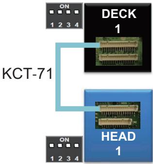
Figure 18-12 Single Deck Single Head Remote Mount
