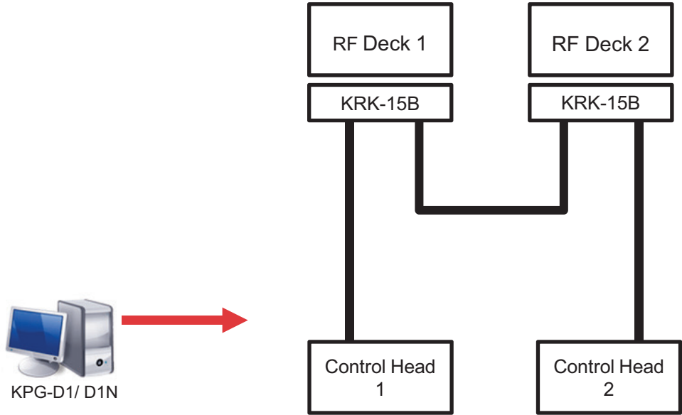
Figure 18-56 Dual RF Deck/ Dual Control Head (FPU Setting)
