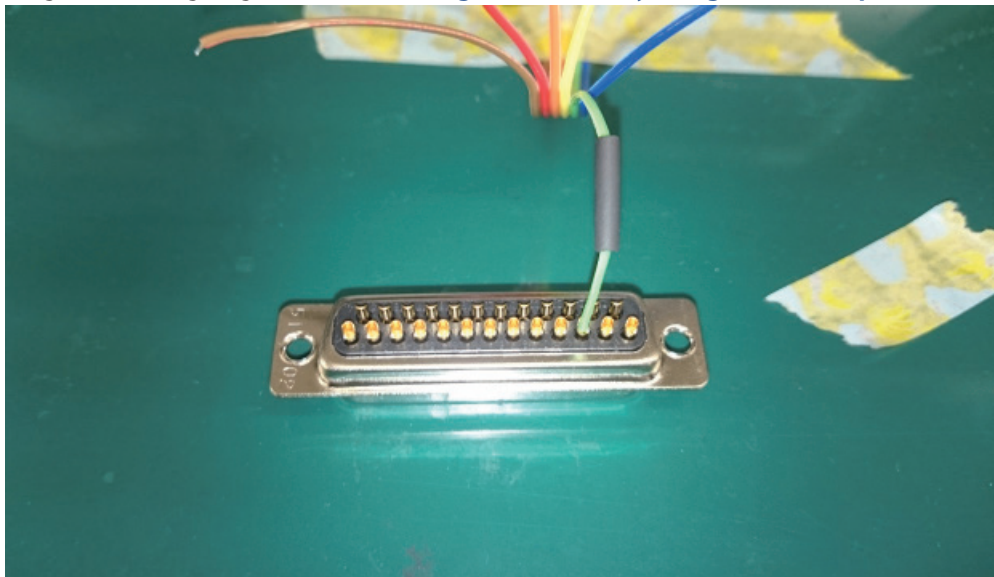
Figure 17-94 Cable Connection 1
