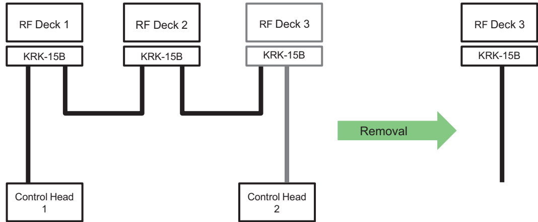
Figure 18-52 Removal of RF Deck 3/ KCT-71
