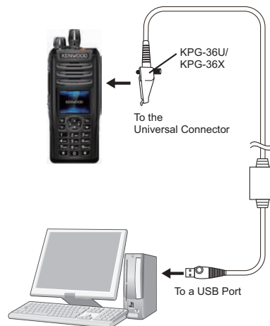
Figure 2-2 Connection of the Transceiver (Portable) and a PC
