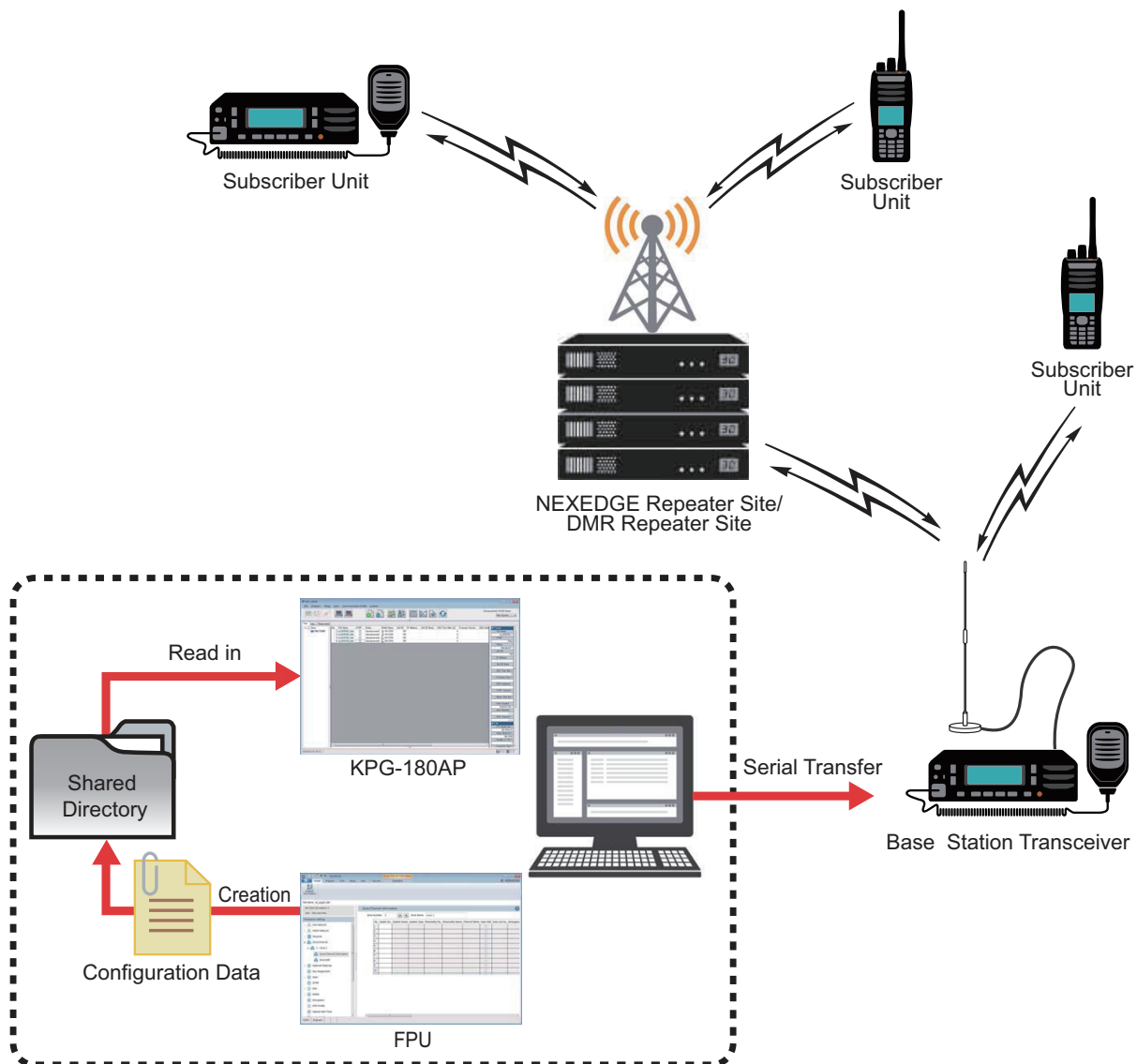
Figure 2-6 Example of the System Structure
