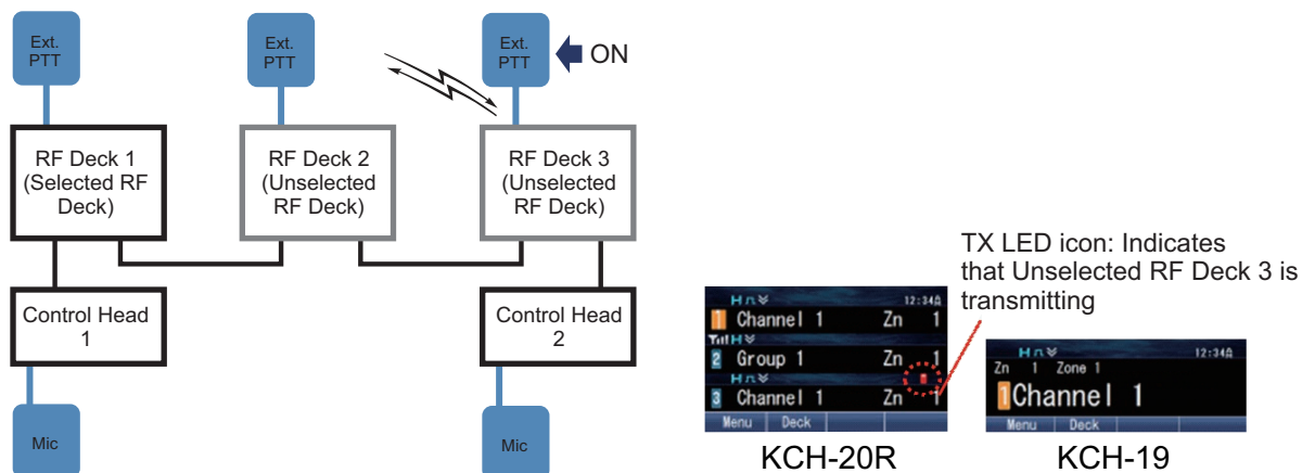
Figure 17-33 Case 2: Transmitting by the External PTT connected to a D-sub connector
