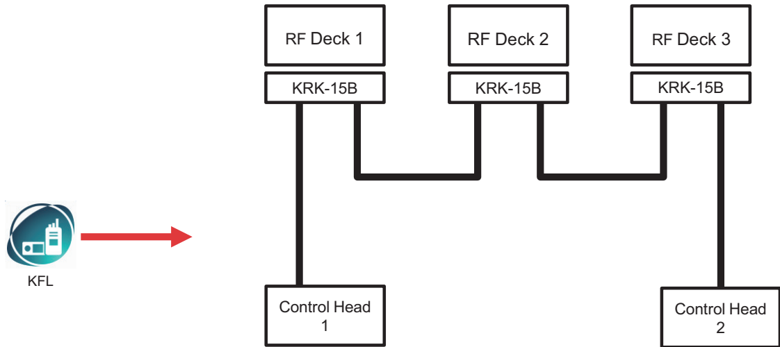
Figure 18-22 Triple RF Deck/ Dual Control Head (Firmware Setting)
