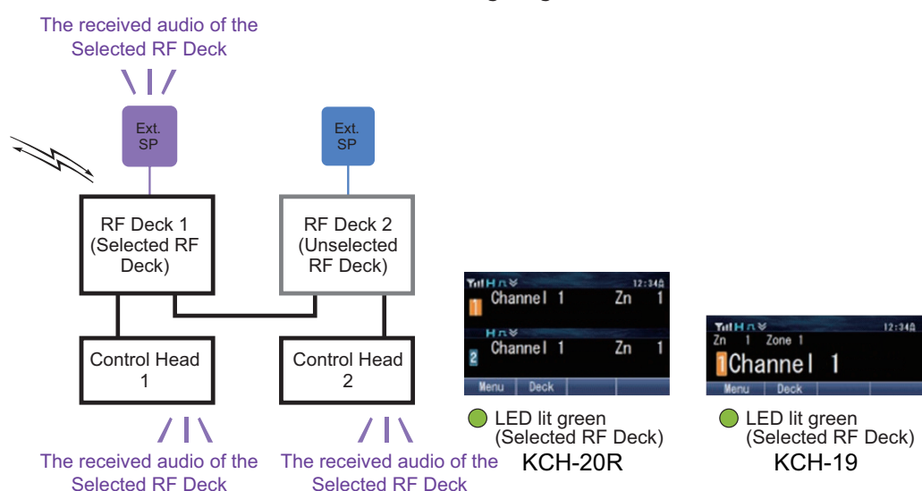
Figure 17-29 Case 1: Received by the Selected RF Deck
